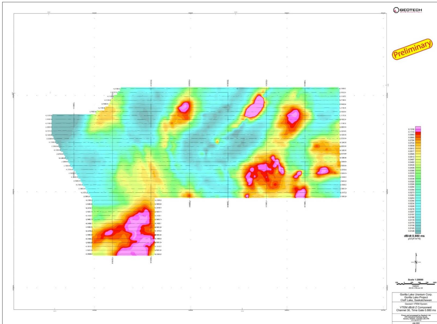
Figure 13 dB/dt Z Component Channel grid
