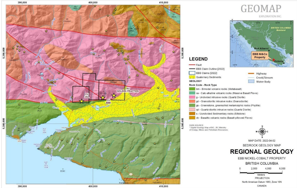
Figure 6: Regional Geology
