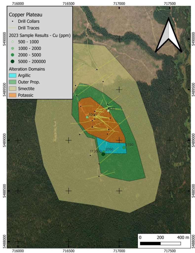
Figure 3 Zonation Map of Alteration Types at the Copper Plateau Project.
