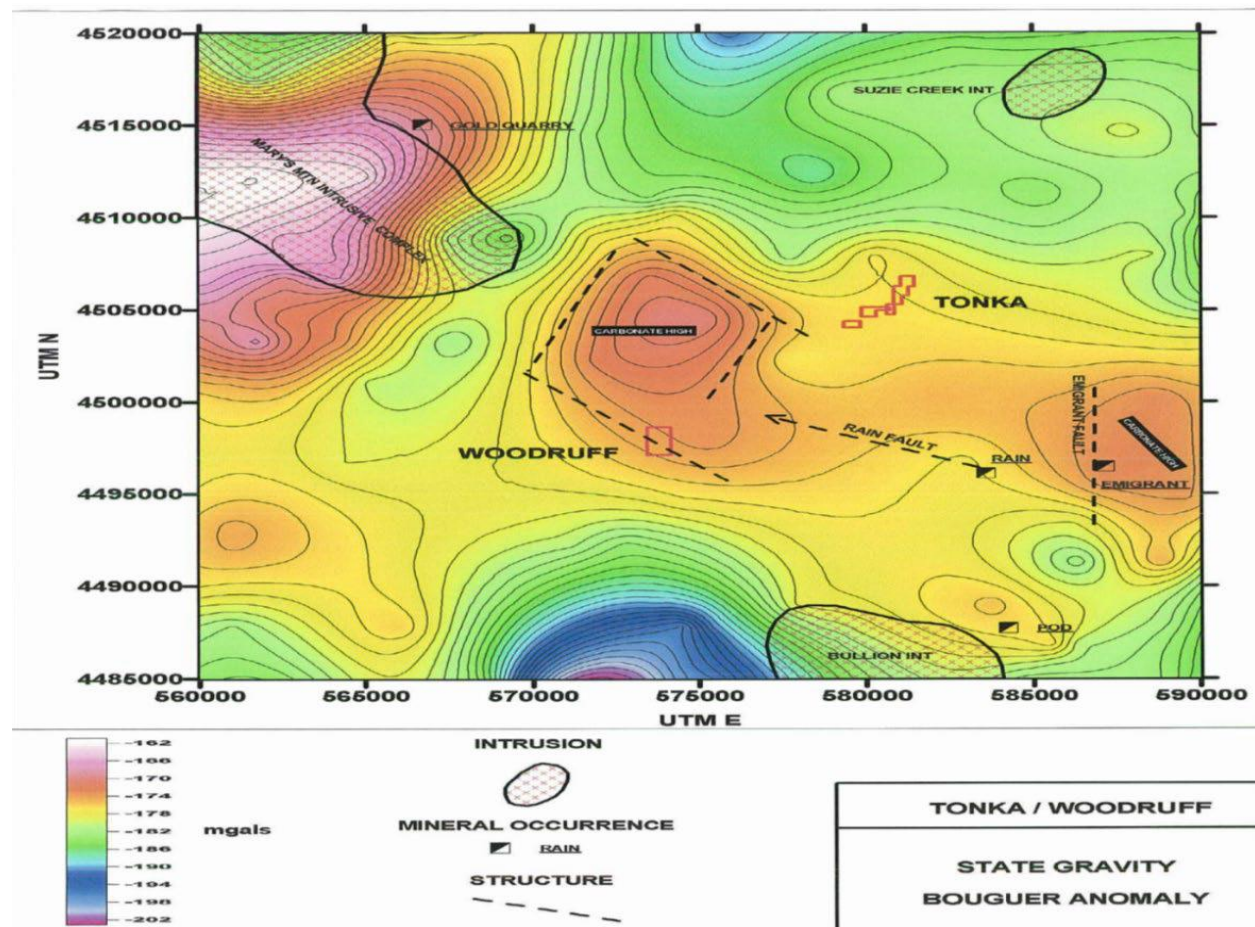
Contour map of Bouguer gravity survey results
