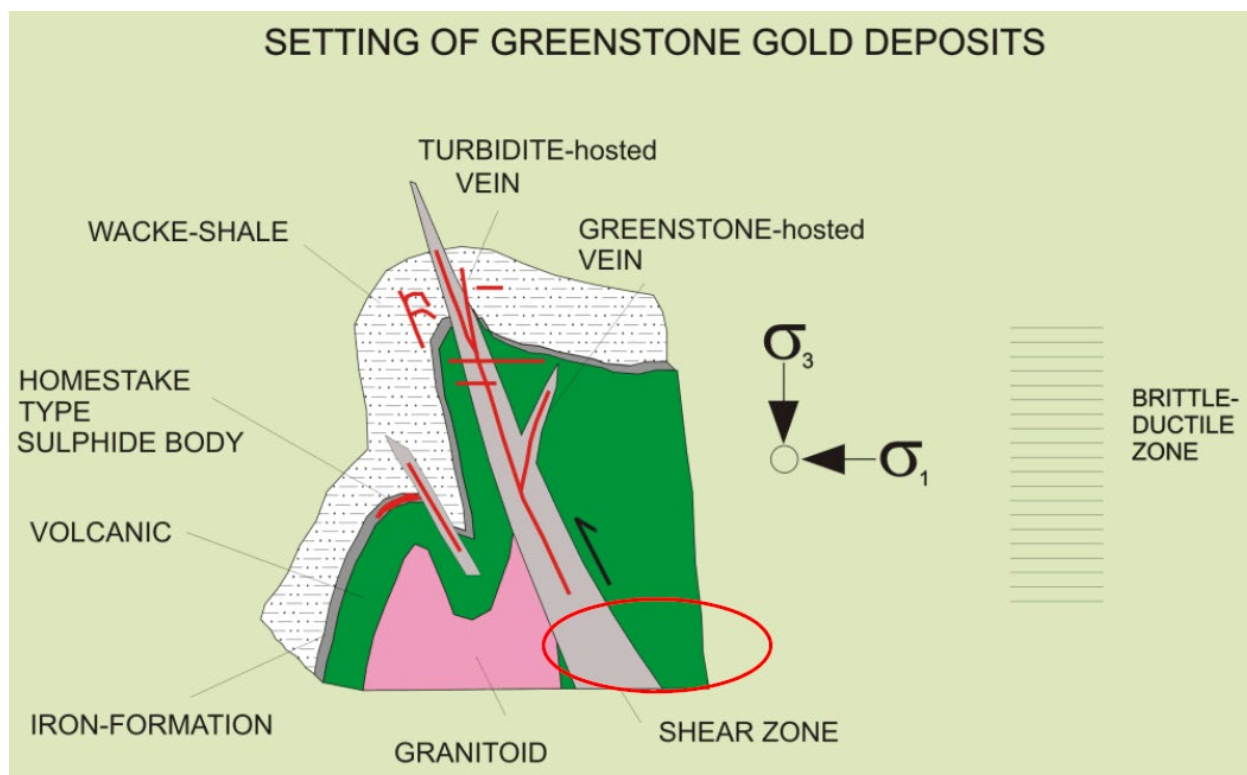
Figure 8-1: Setting of GQC Gold-Vein Deposits (Dube and Gosselin, 2007)
