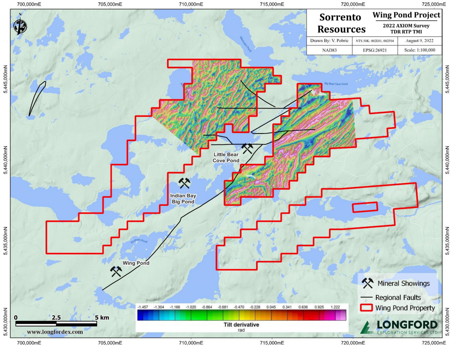
Figure 9-6: Wing Pond Property TDR RTP TMI.
