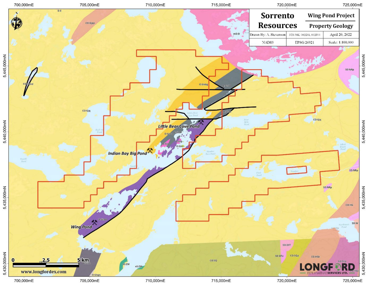
Figure 7-5: Wing Pond Local Property Geology.
