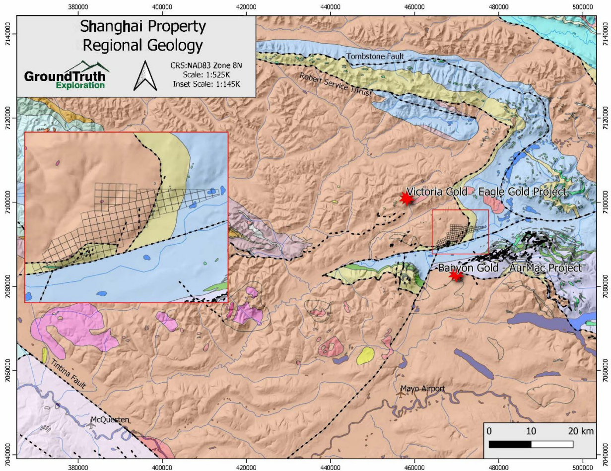
Figure 7.1: Regional Geology
