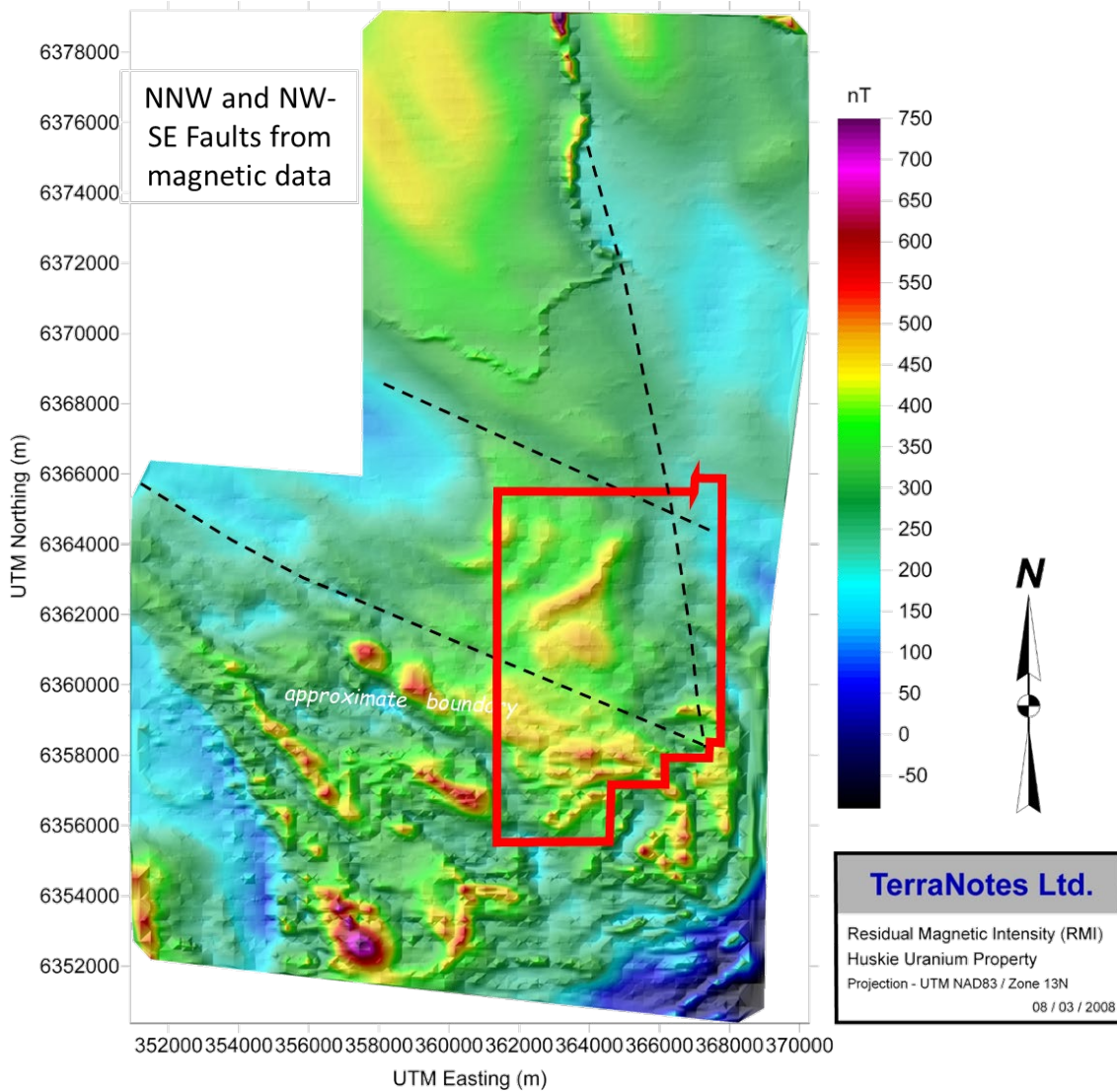
Figure7: Magnetic structures on Property.
