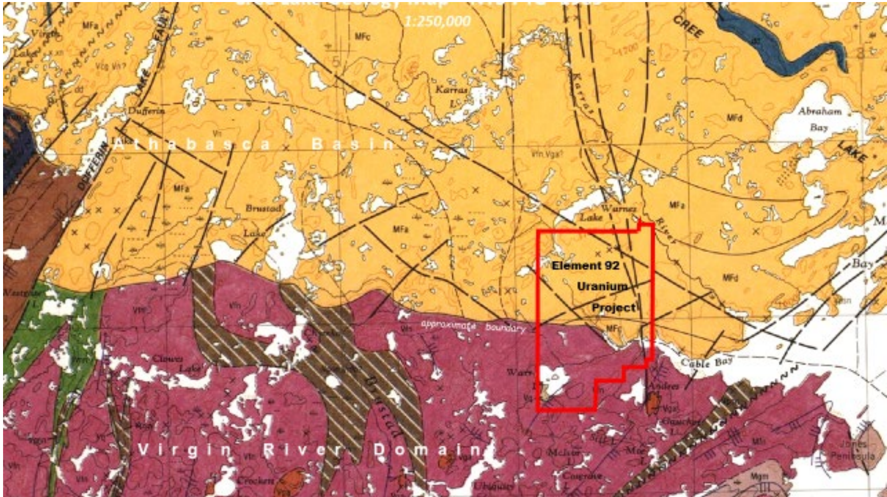
Figure 5: Property Geology and Stratigraphic Column.
