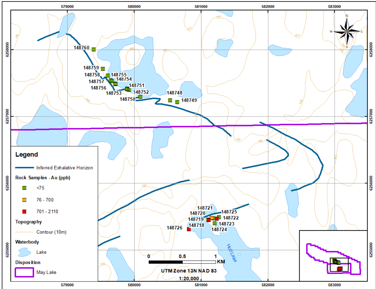
Figure 10- 2021 Rock Samples – Au (ppb)
