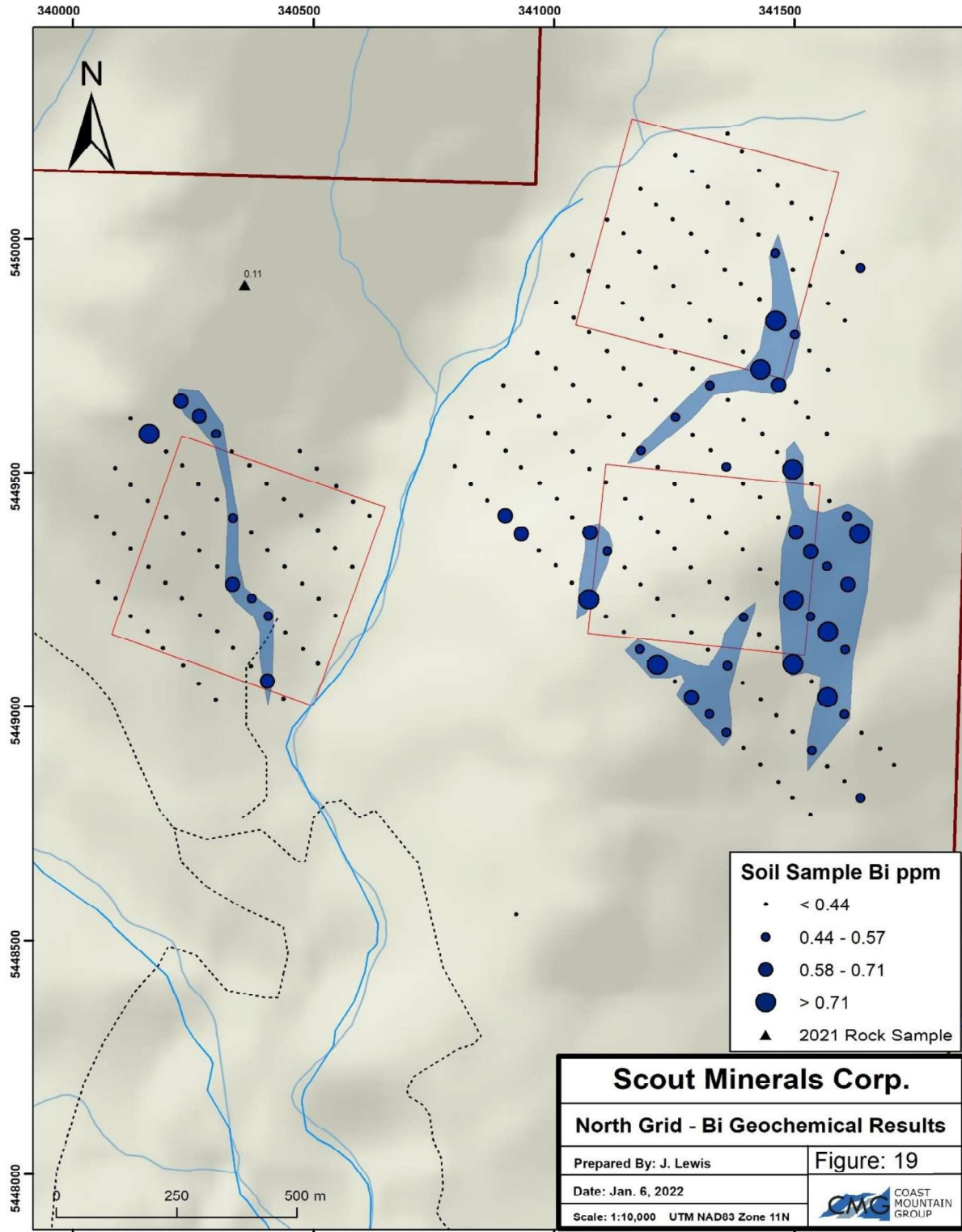
Figure 19 - North Grid Bi Geochemical Results
