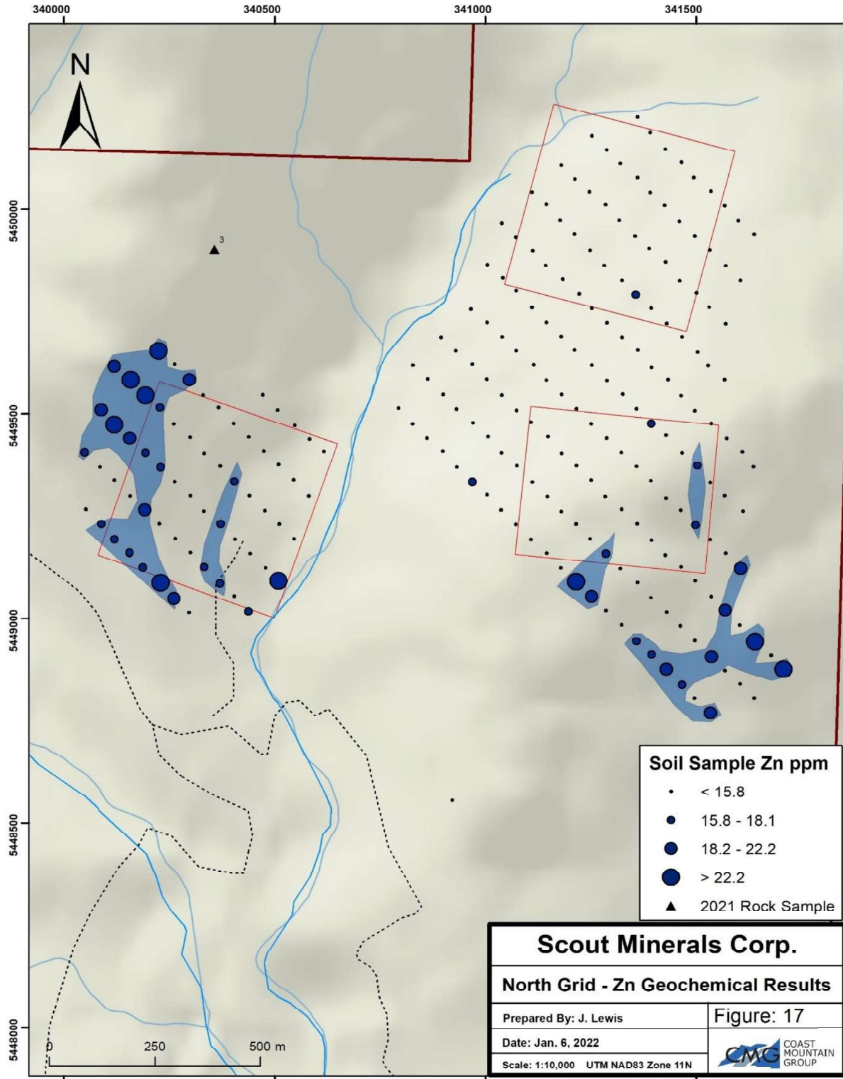
Figure 17 - North Grid Zn Geochemical Results
