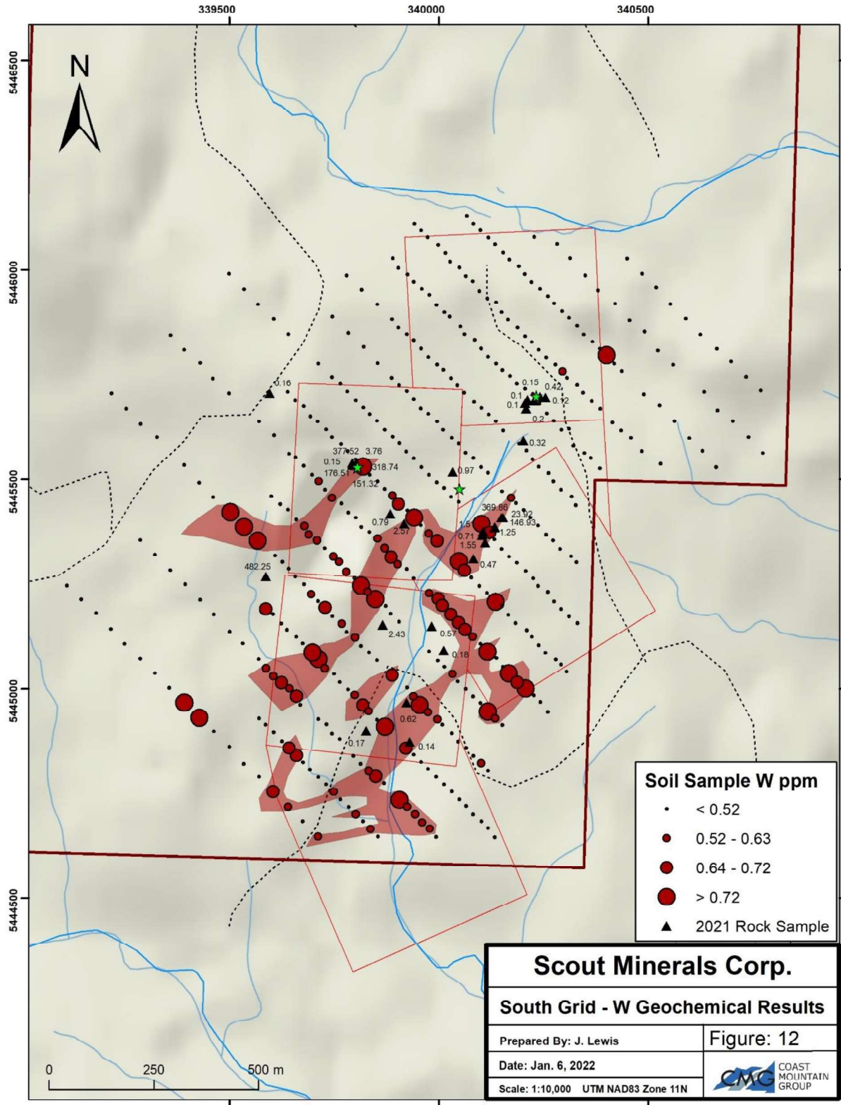
Figure 12 - South Grid W Geochemical Results
