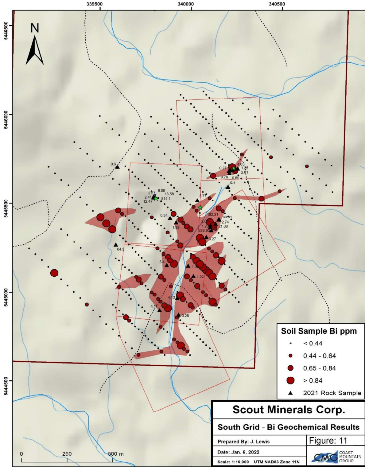
Figure 11 - South Grid Bi Geochemical Results
