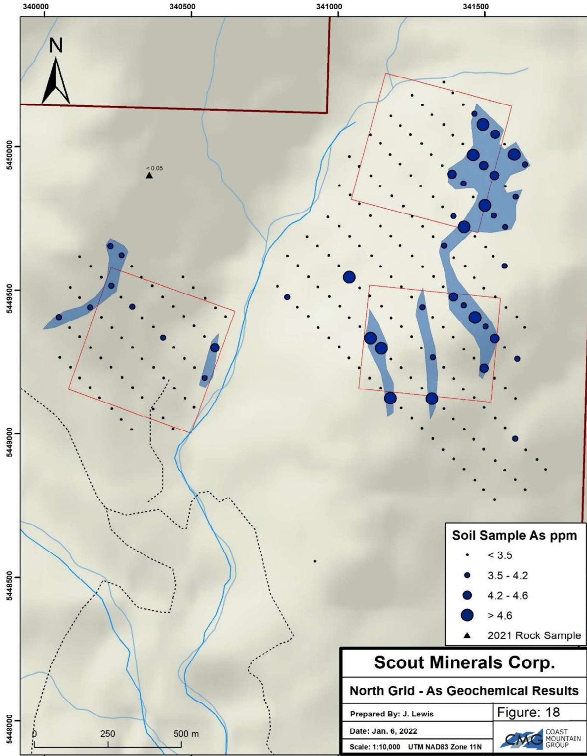
Figure 18 - North Grid As Geochemical Results
