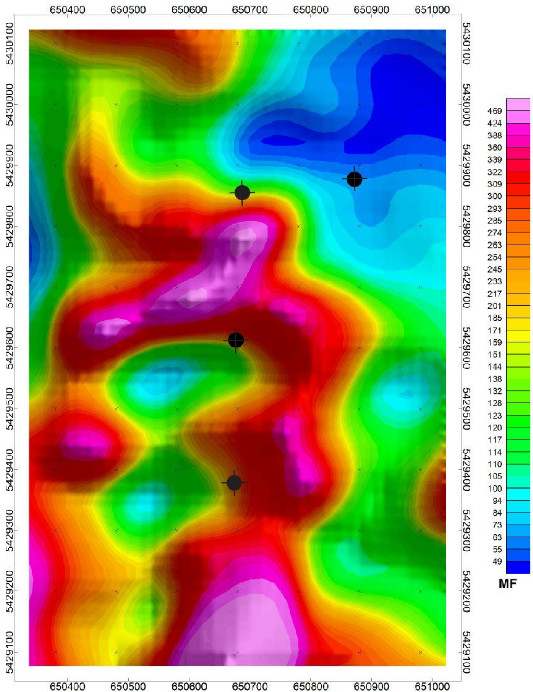
Xcite Resources Inc. IP Survey - DASVision Metal Factor - 250 m Level Figure 9.1
