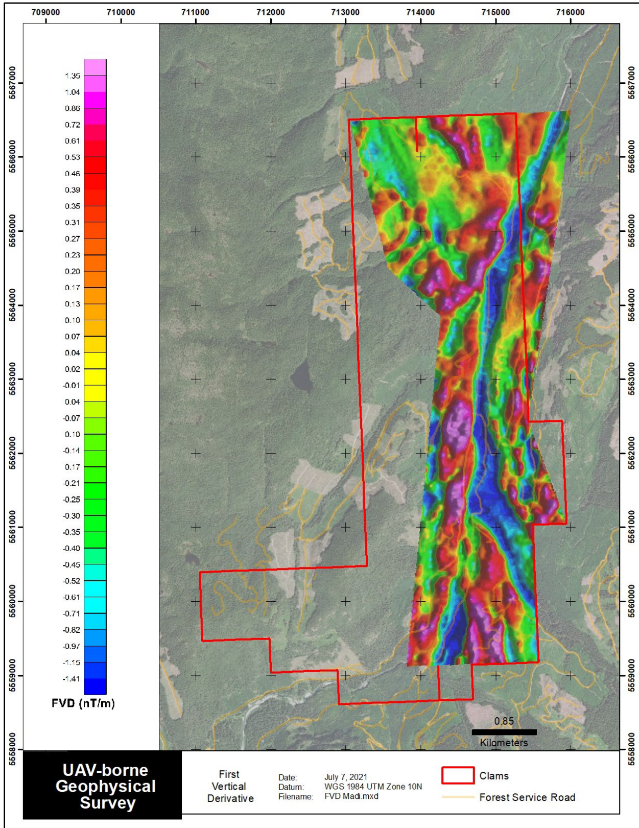
Figure 12: UAV-borne geophysical survey
