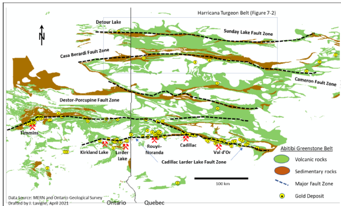
Figure 9. Abitibi Greenstone Belt Regional Geology
