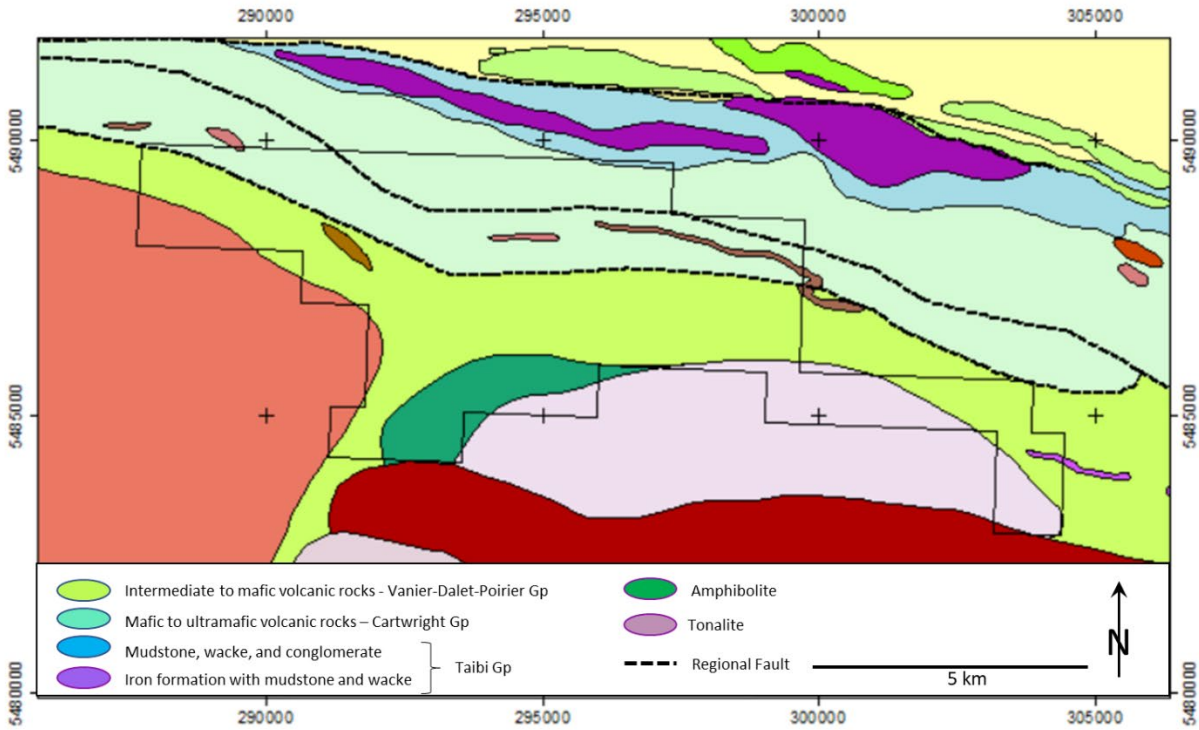
Figure 11. Property Geology
