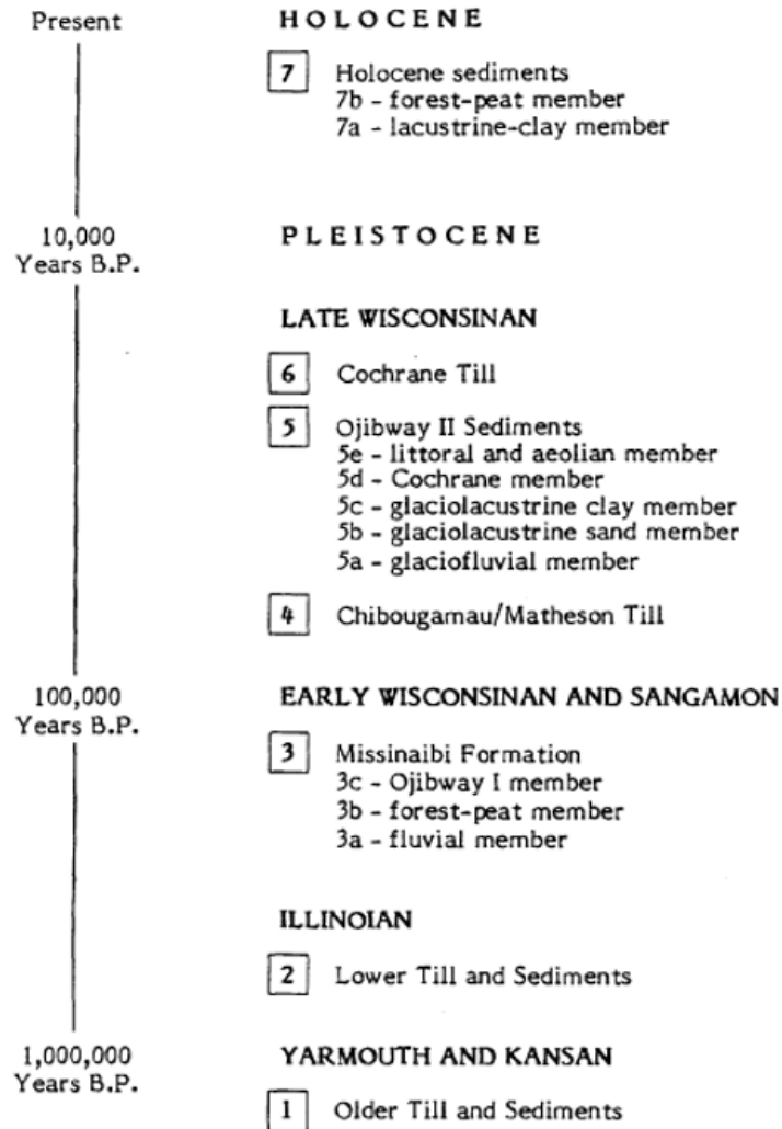
Figure 13. Quaternary Formations Of The Abitibi
