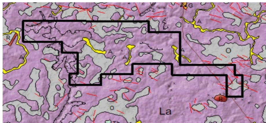
Figure 11. Property Geology
