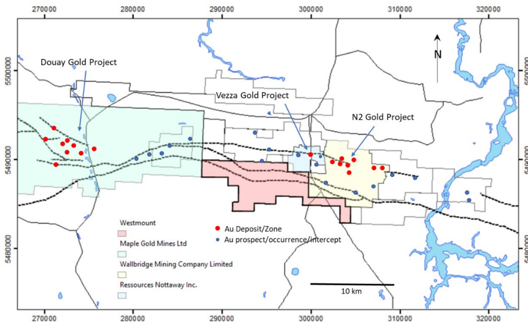
Figure 17. Adjacent Properties
