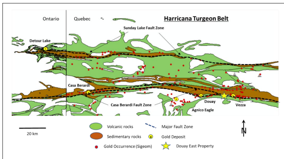
Figure 10. Local Geology
