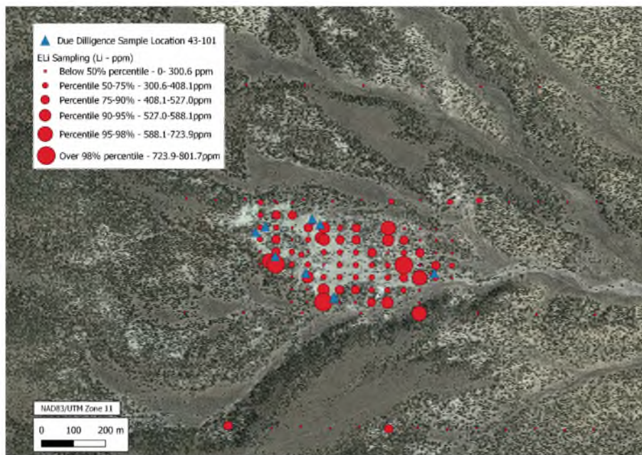
Figure 4. Presentation of the results for the lithium-in-soil (133 samples), Li-in-rock (2019, 16 samples) and the due diligence QP sampling (2021; 9 samples, blue triangles) over the ELi property. The highest values generally corresponded with outcropping Li..
