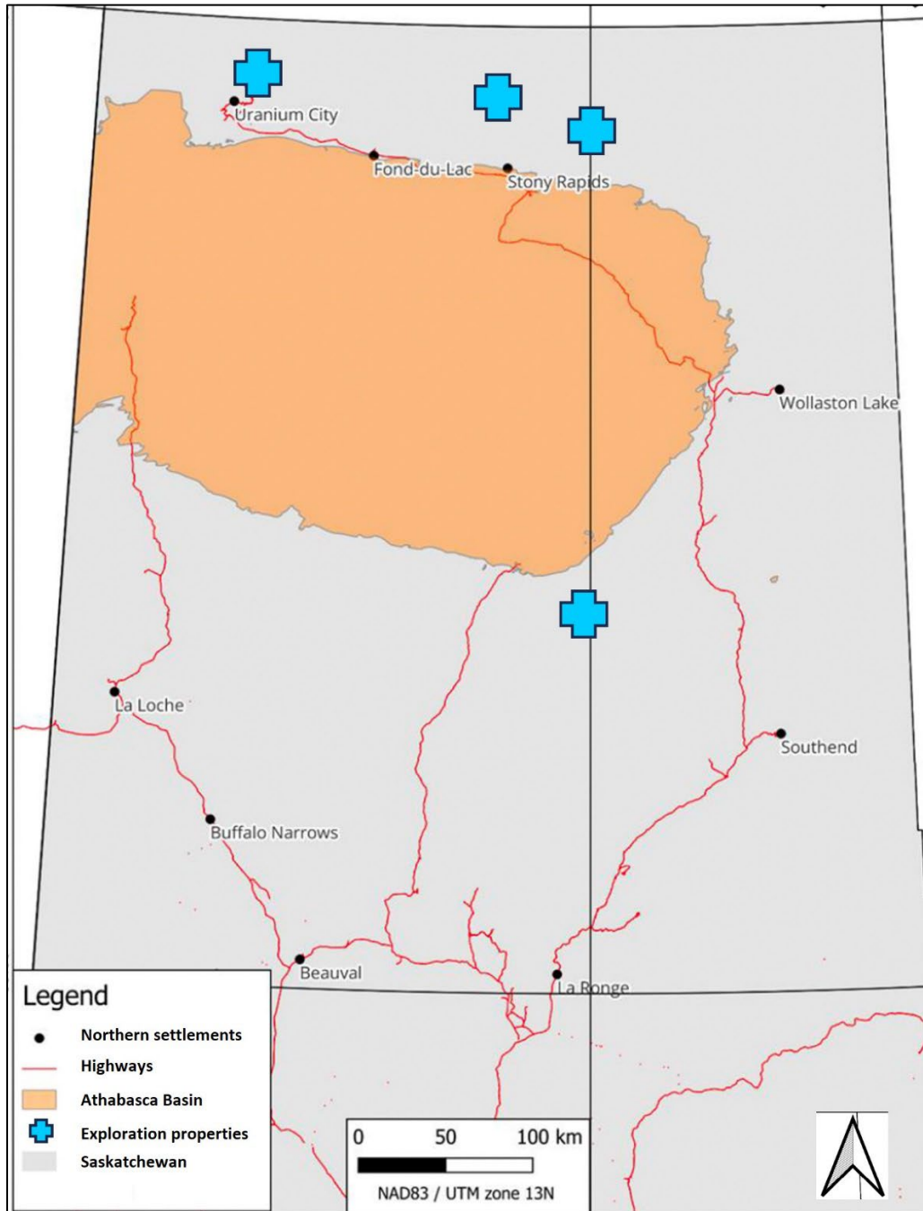
Figure 1. Regional map of northern Saskatchewan, Canada which is one of the world's leading sources of high-grade uranium and supplies about 20% of the world's uranium. The blue symbols illustrate locations of the four optioned exploration properties totalling 596 km 2 in the context of the world-famous Athabasca Basin, a Paleoproterozoic siliciclastic depo-centre ( click here to view image ).
