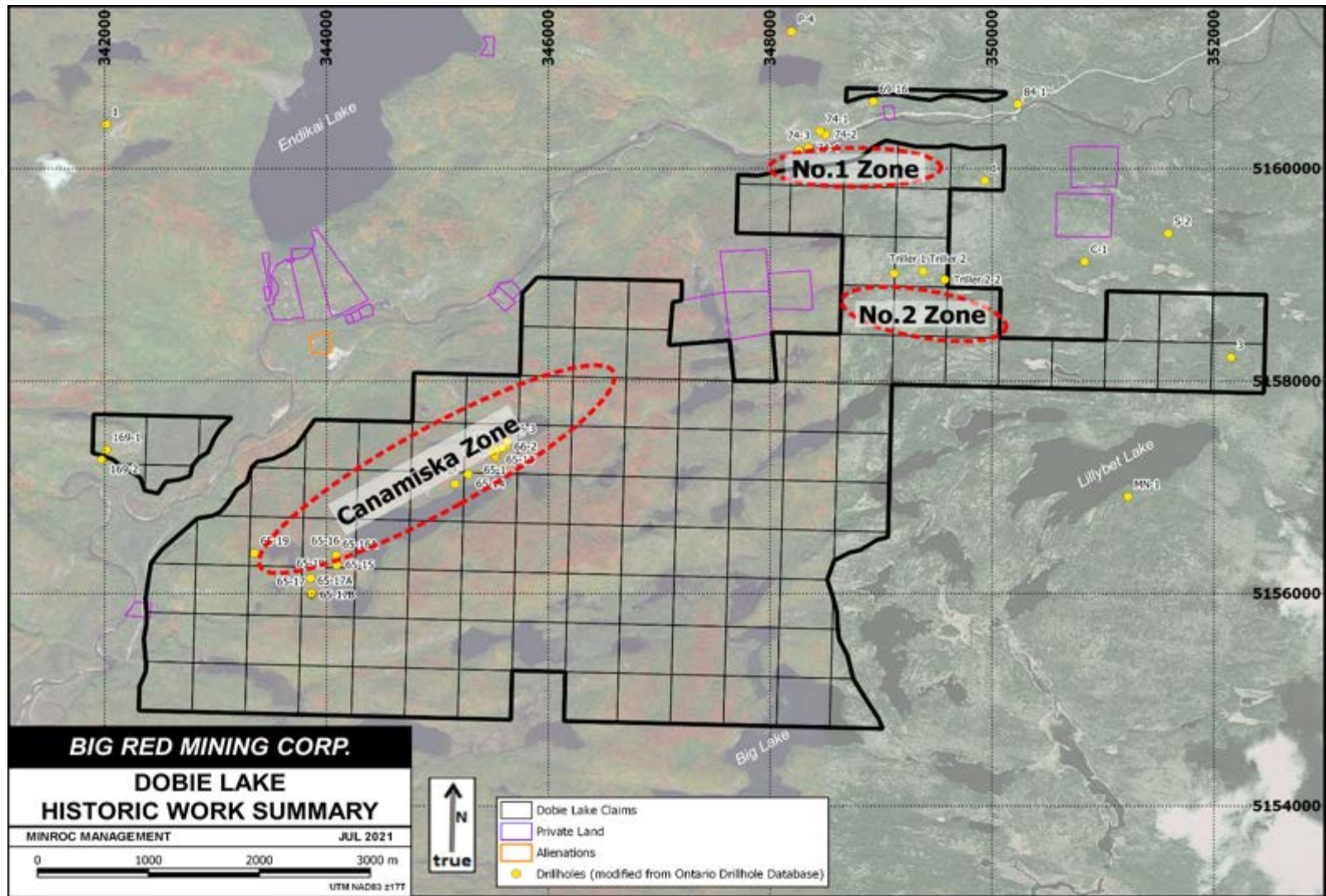
Figure 3 Summary of Historic Work on the Dobie Lake Property. Drillhole locations are modified from Ontario Drillhole Database after an assessment file review
