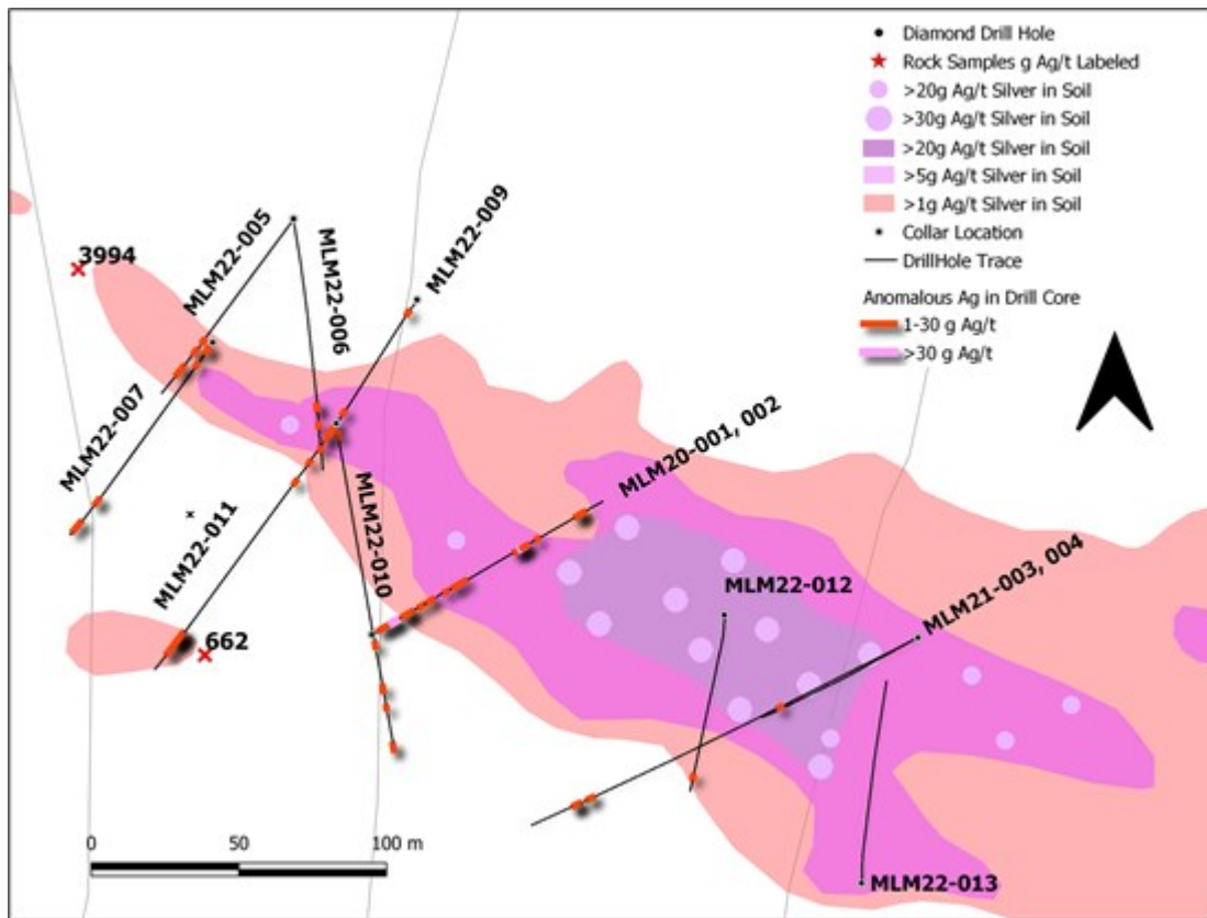
Figure 1. Carlin West silver in soil anomaly showing drill holes completed during 2020, 2021 and 2022
