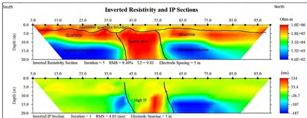
Figure 9.19: MLM5 Inverted Resistivity and IP Sections, Carlin-Roop Property
