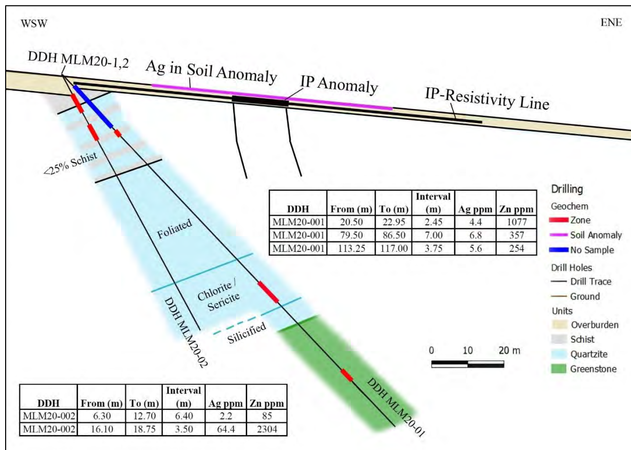
Figure 10.2: 2020 Drill Profile
