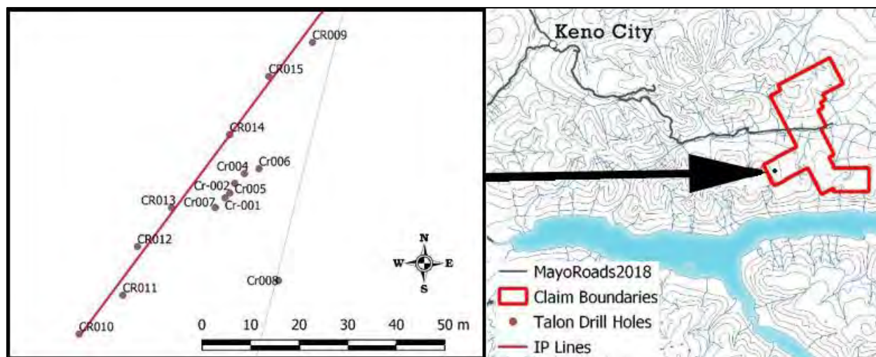
Figure 9.18: KAI IP Line and Talon Drill Hole Locations
