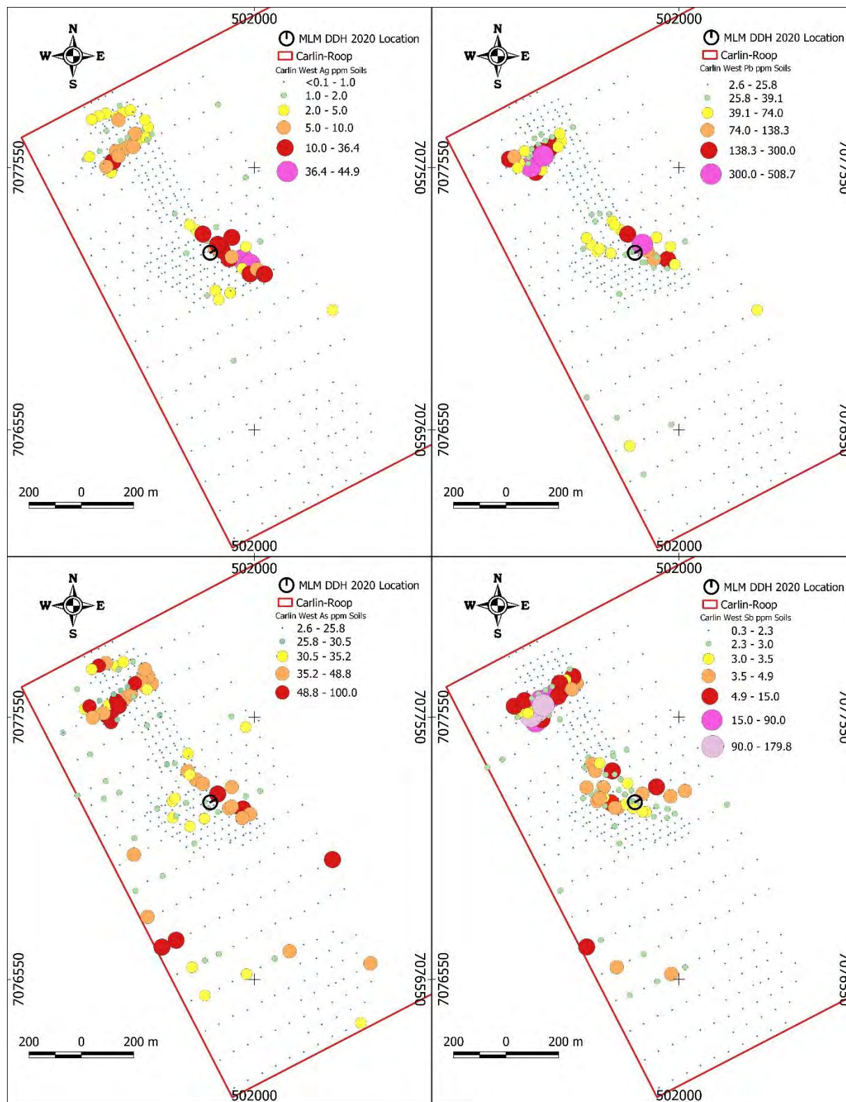
Figure 9.12: Carlin West All Soil Survey - Compare Ag Pb As Sb
