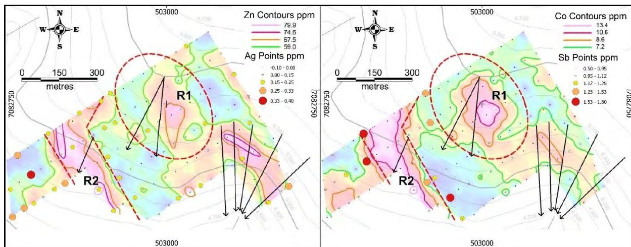
Figure 9.7: 2014 Soils Roop North R2, Zn with Ag and Co with Sb
