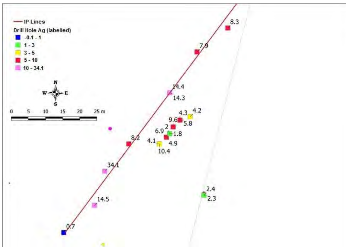
Figure 9.20: Carlin West Backpack Drill Holes with Ag Analysis over IP Line
