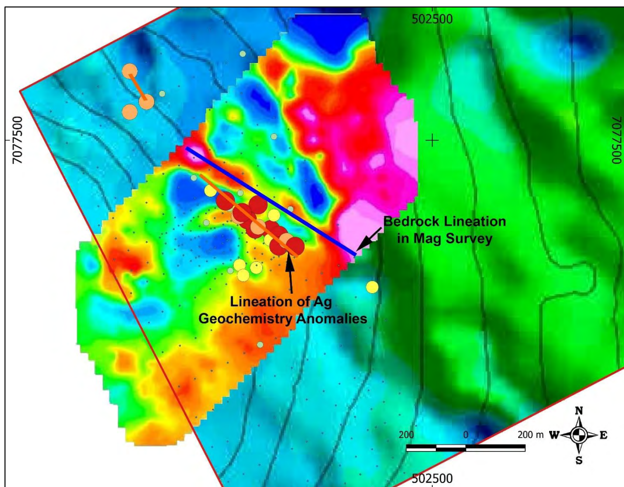
Figure 9.17: Carlin West Ground Total Magnetic Intensity over 2012 Airborne TMI
