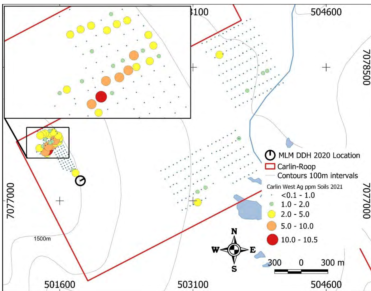
Figure 9.11: Carin West 2021 Ag in Soils ppm
