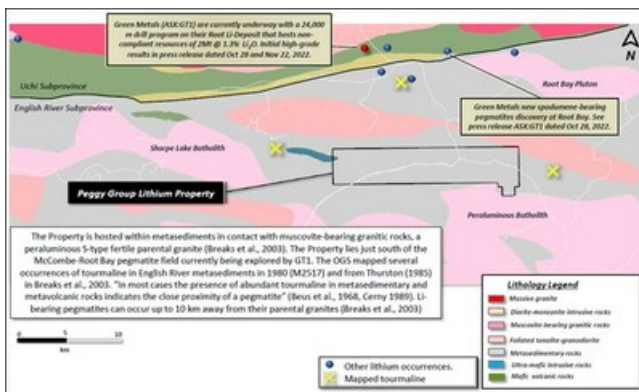
Figure 3 – Regional Geology (CNW Group/Beyond Minerals Inc.)
