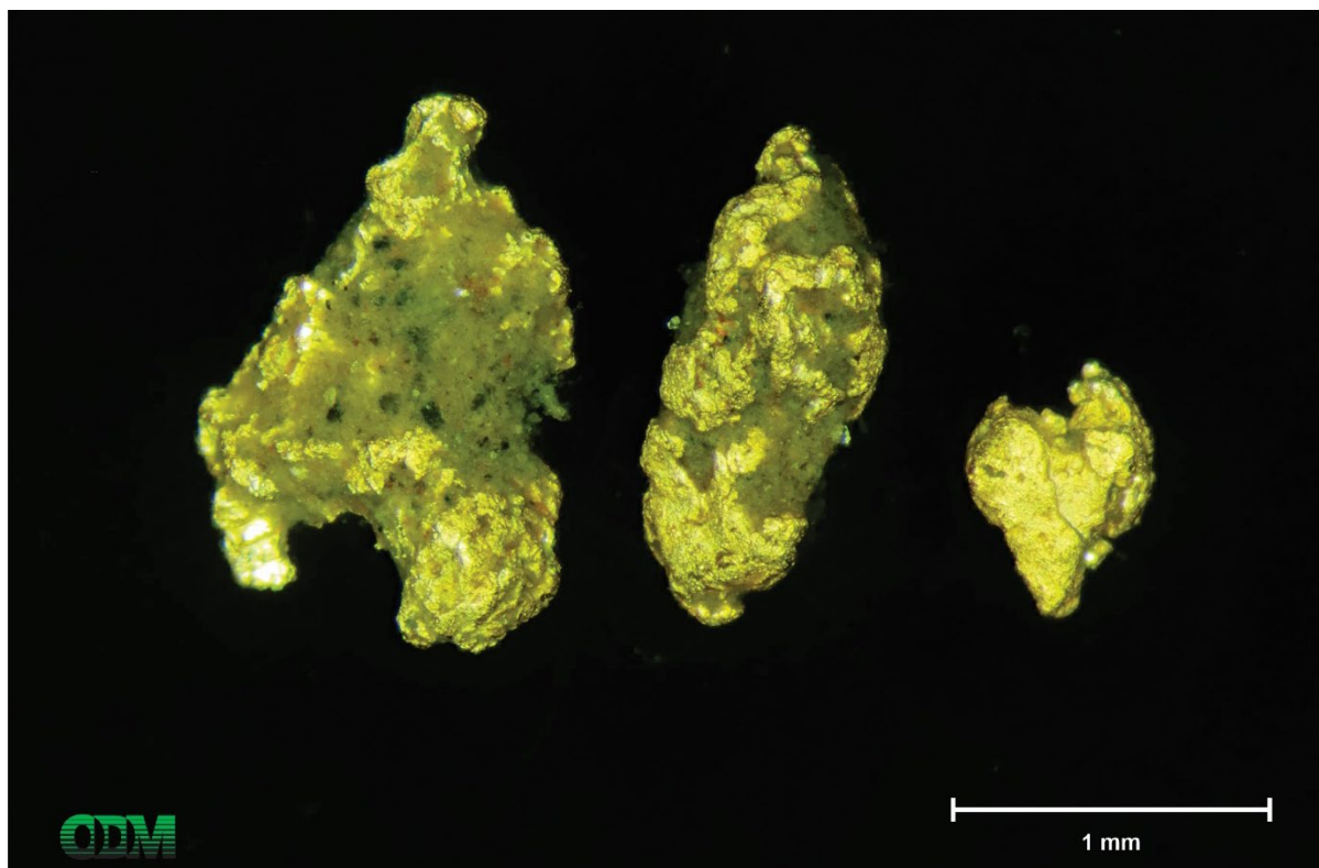
Figure 1: Photomicrograph of selected modified and reshaped gold grains from SG-22-TIL-04. Note scale bar lower right.
