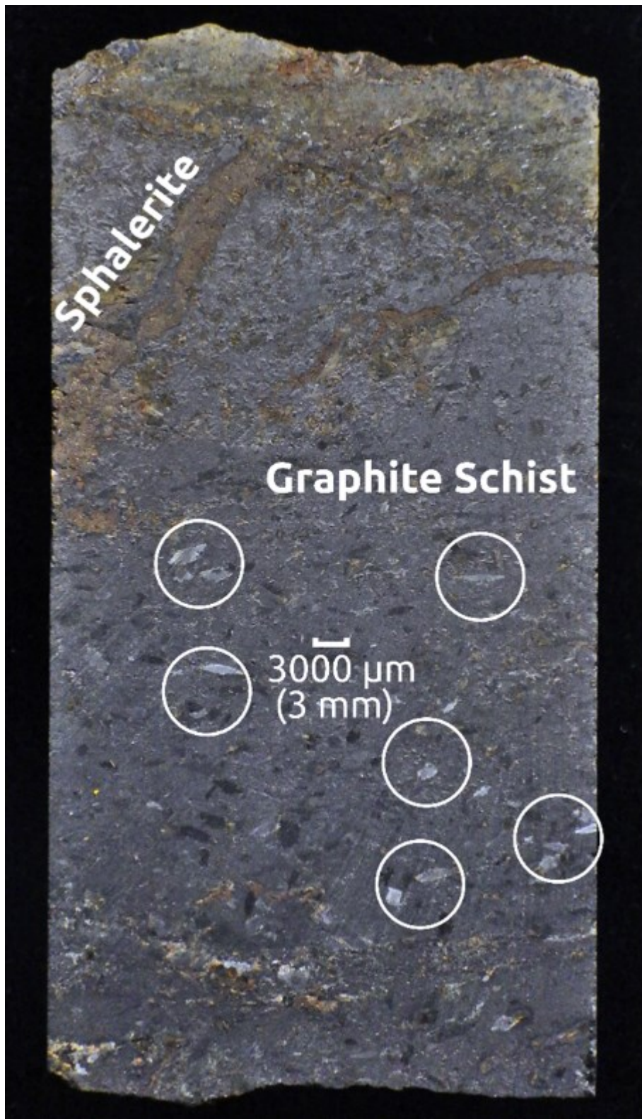
Figure 3 – Jumbo Graphite flakes identified in DDH#1 (19.80m) included in Composite Sample #1 of the QEMSCAN Study. (click the image for an enlarged view)
