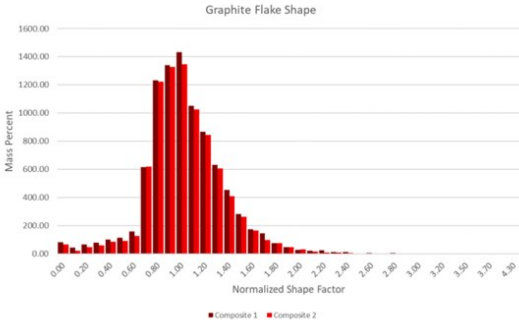
Figure 5 - Distribution of graphite flake shape vs particle count
