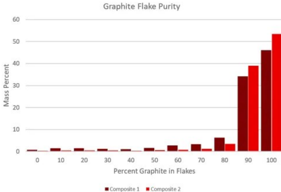
Figure 6 - Graphite Flake Purity categorized in 10% increments
