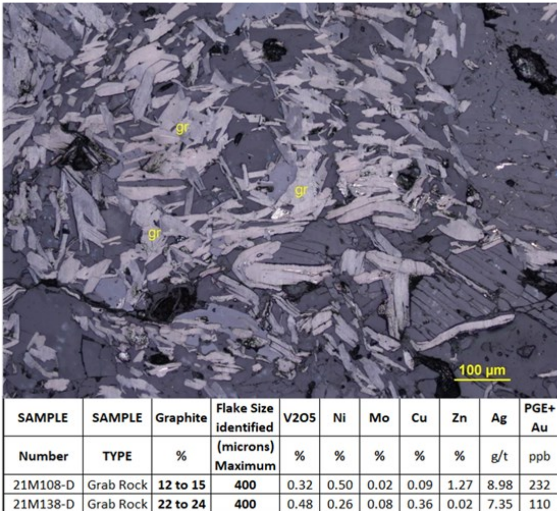
Figure 4 - Surface Sample 21M108 Randomly oriented lamellae of graphite (gr) define an irregular cluster within the quartz. Plane-polarized transmitted light. (click the image for an enlarged view)
