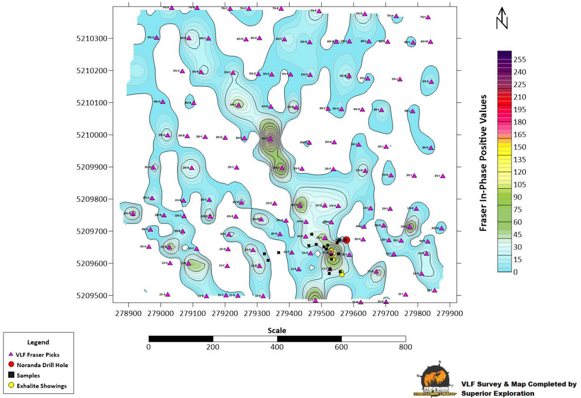
Figure 1: Location of Buck Lake VLF-EM Anomaly trending NW-SE and highlighting stronger anomalies in two areas. The location of the Noranda Drill hole (with massive sulphide zones) is shown intersecting the southern anomaly. The samples collected are also shown.
