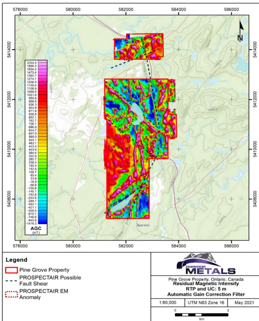
Ground Magnetics Survey – Residual Magnetic Intensity Figure
