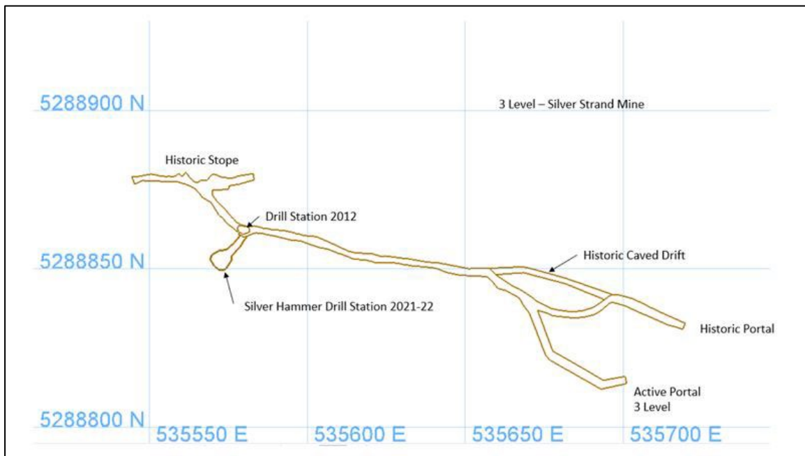
Figure 9-3: Plan view of the No. 3 Level in the Silver Strand Mine
