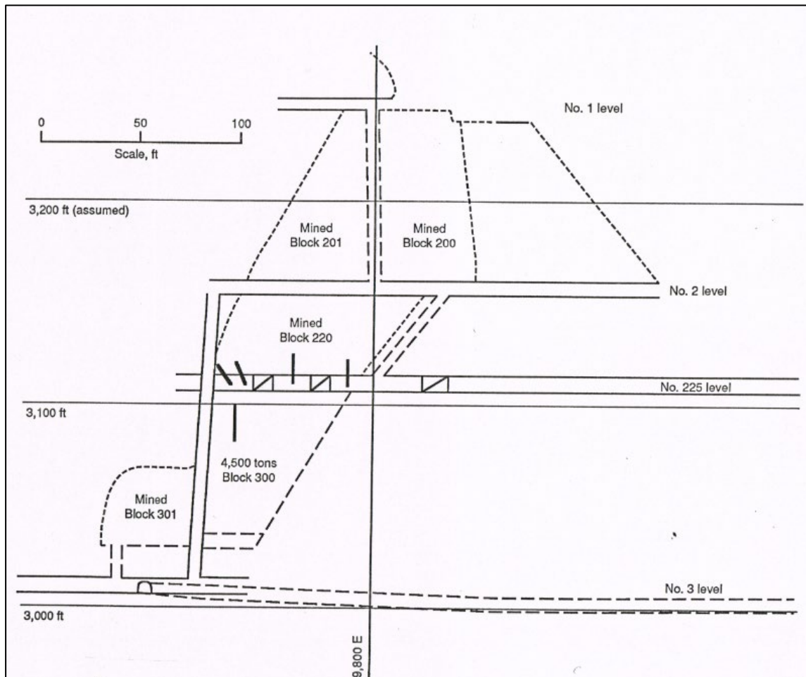
Figure 6-3: Cross Section of the Silver Strand Mine, 1992, showing the location of drillholes (thicker black lines) in the No. 225 adit
