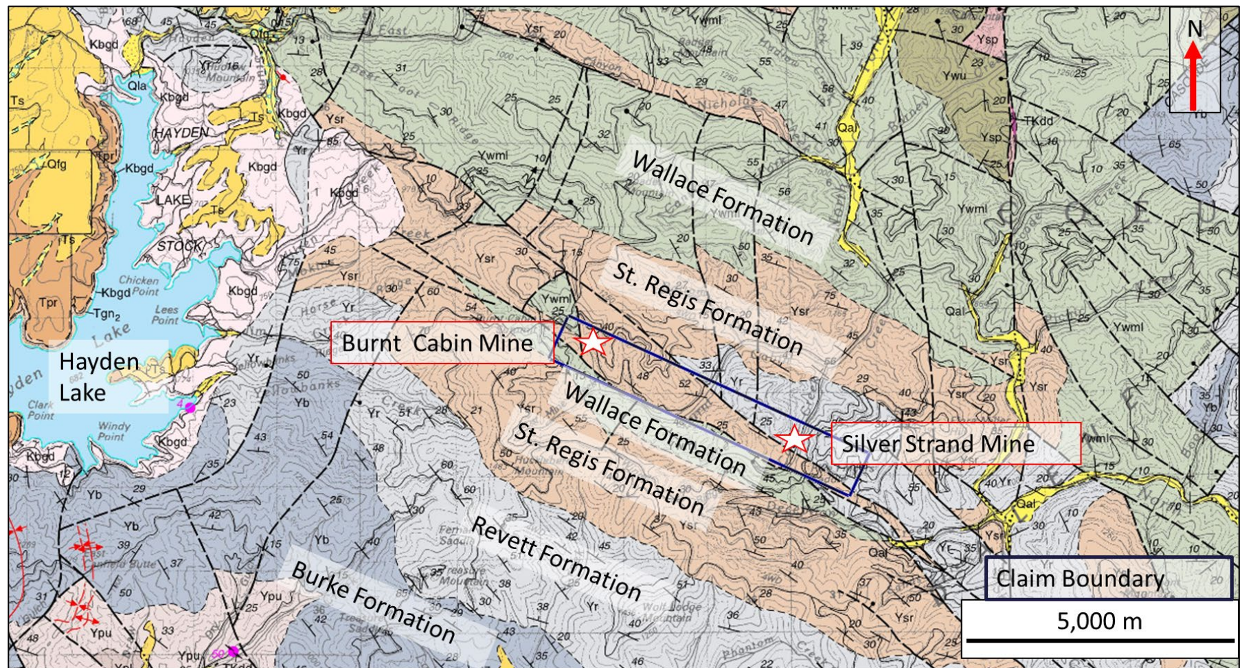
Figure 7-3: Local Geology Setting for Silver Strand Area
