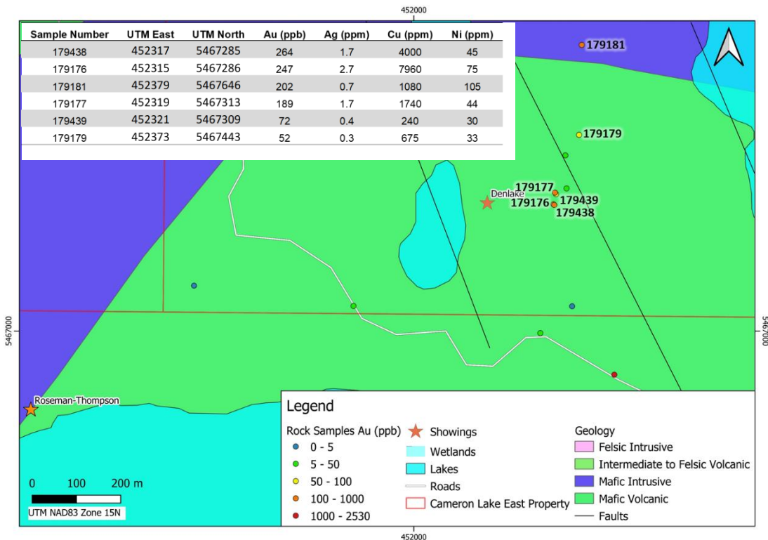
Figure 13. Samples around the Denlake Showing (C. Hudek, 2020)..
