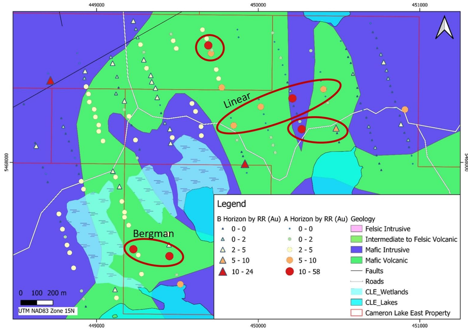
Figure 6. Soil results by Au response ratio. Values above 5 are considered anomalous for gold (orange and red samples) (C. Hudek, 2020)..
