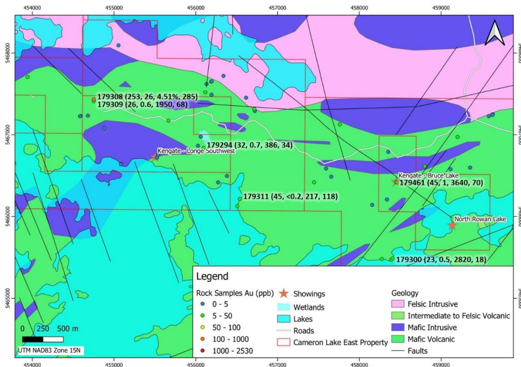
Figure 15. Rock highlights from the east side of Rowan Lake. Value listed beside rock grab samples are (Au ppb, Ag ppm, Cu ppm, Ni ppm) (C. Hudek, 2020)..
