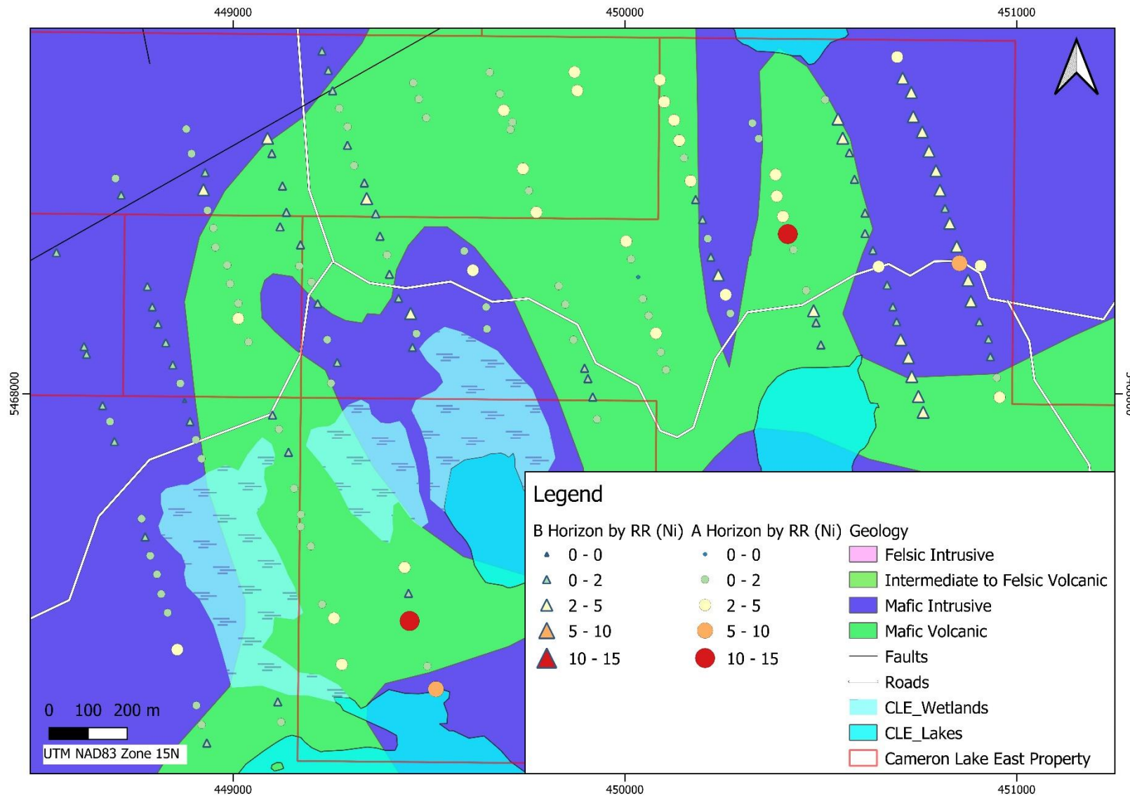
Figure 8. Soil results by response ratio for Nickel. Values higher than 10 are considered anomalous (red samples) (C. Hudek, 2020)..
