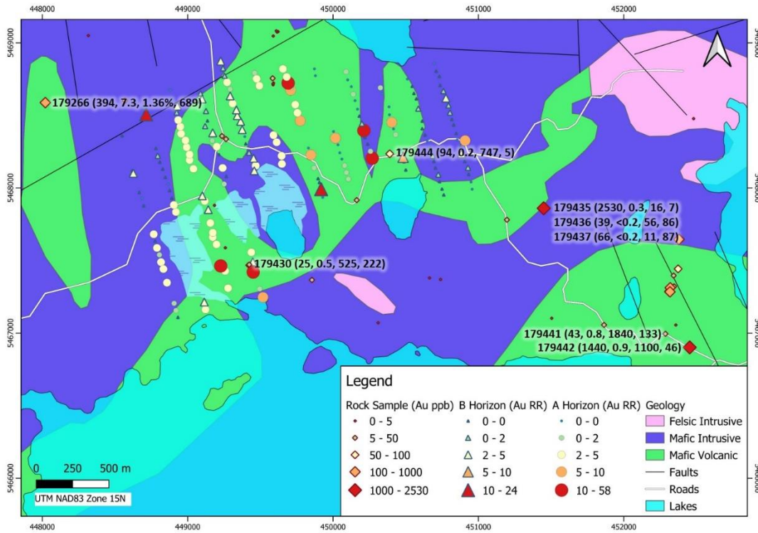
Figure 14. Soil and Rock highlights from the 2020 exploration program with showings. Value listed beside rock grab samples are (Au ppb, Ag ppm, Cu ppm, Ni ppm) (C. Hudek, 2020)..
