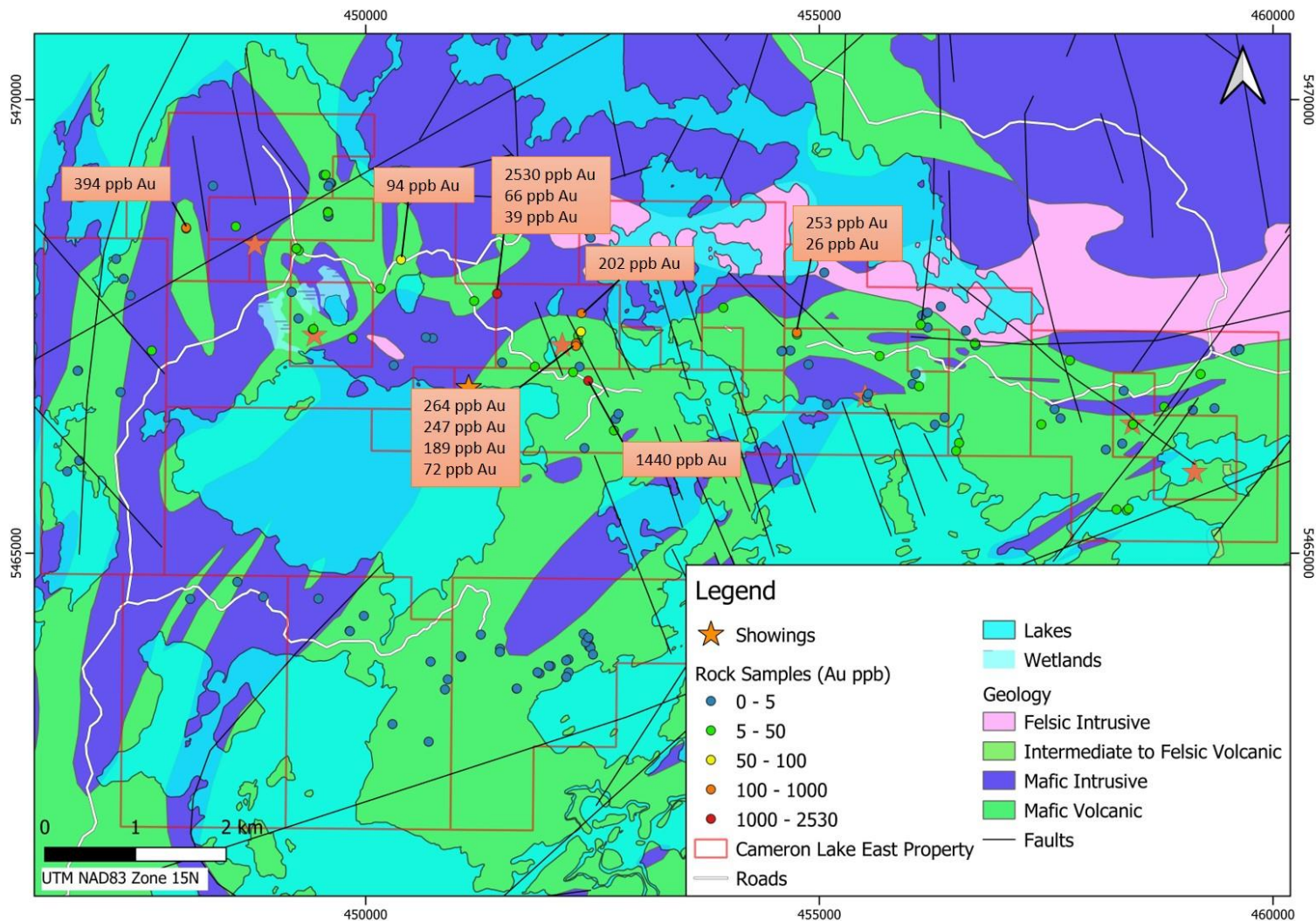
Figure 11. Rock sample highlights (Au ppb) from the 2020 exploration program (C. Hudek, 2020)..
