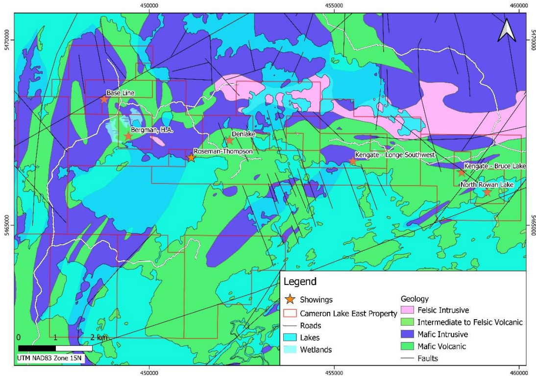
Figure 12. Showings on the current Cameron Lake East Property. List of showings from MDI database from Geology Ontario website (C. Hudek, 2020)..
