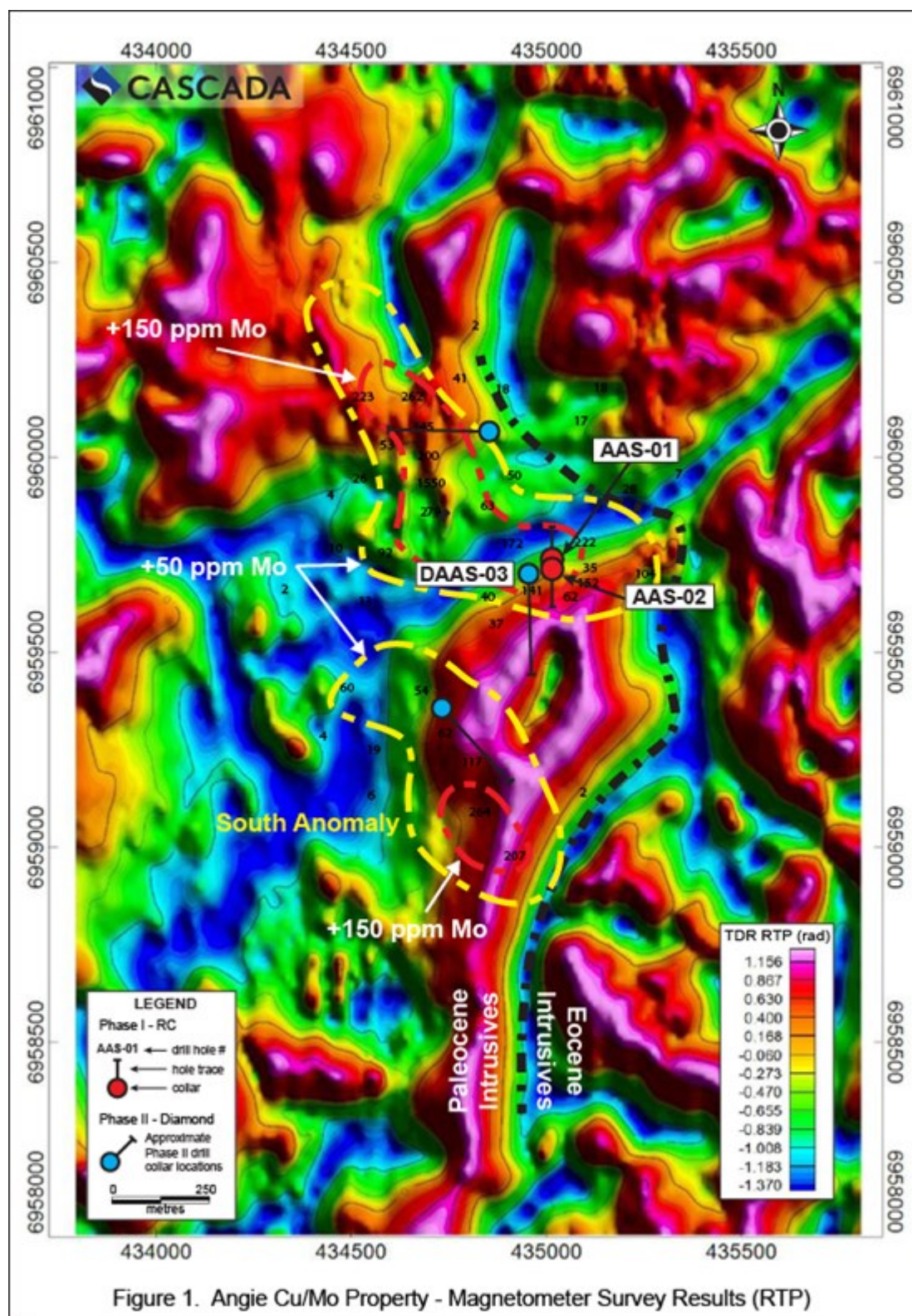
Figure 1. Angie Cu/Mo Property - Magnetometer Survey Results (RTP)
