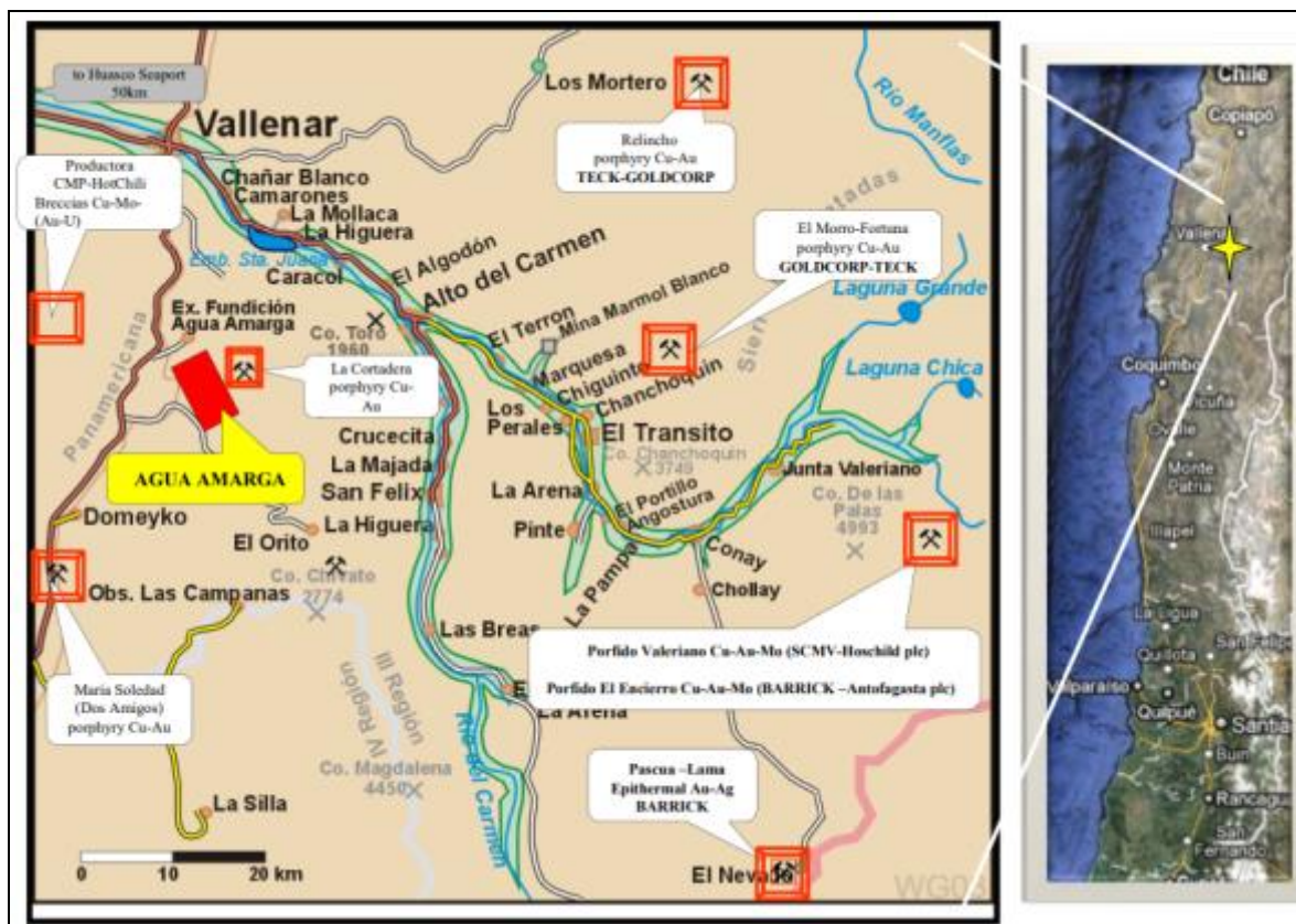
Figure 1 Location of Agua Amarga Property
