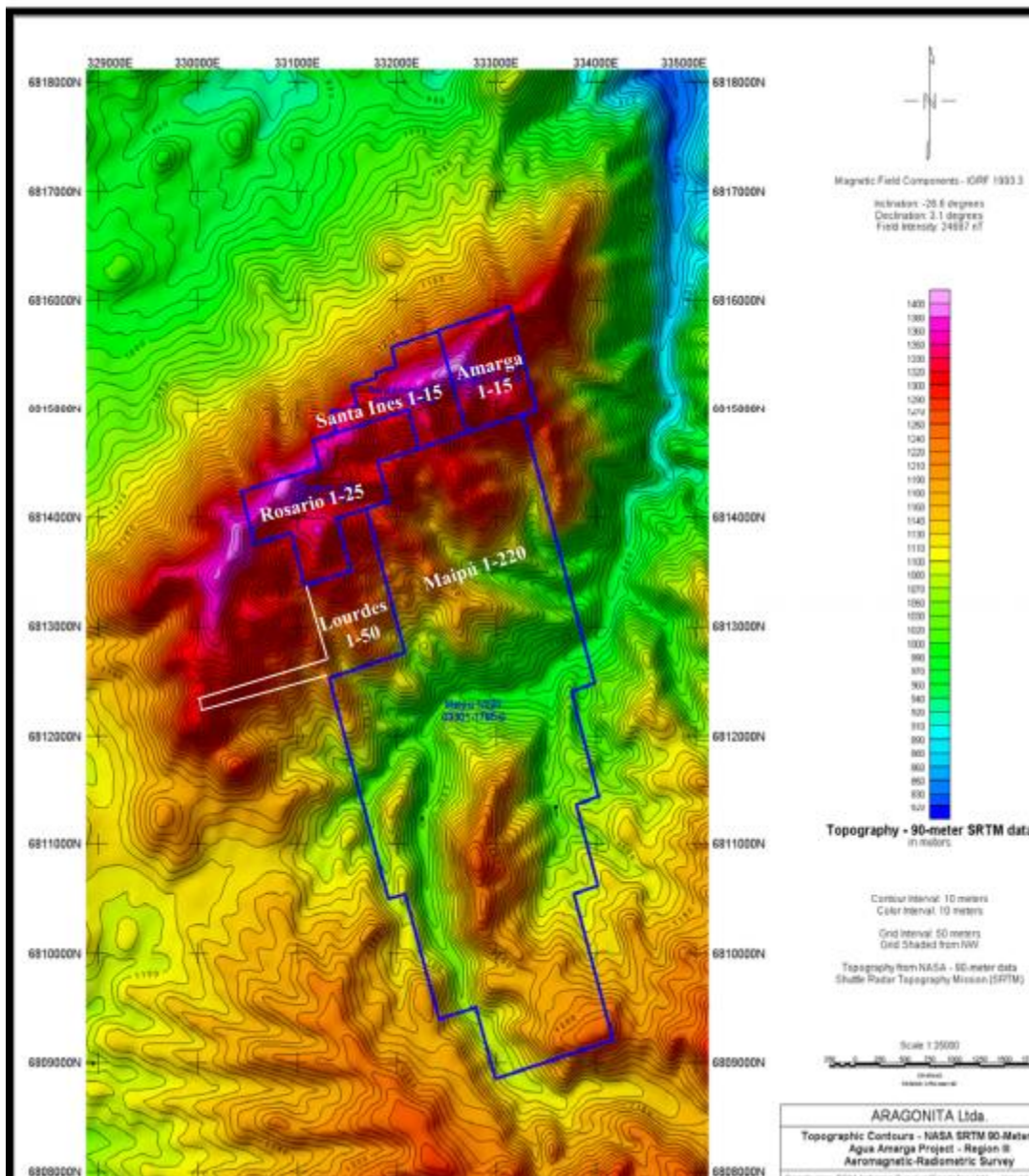
Figure 3 Topography in the Area of Agua Amarga (Araneda, 2017)
