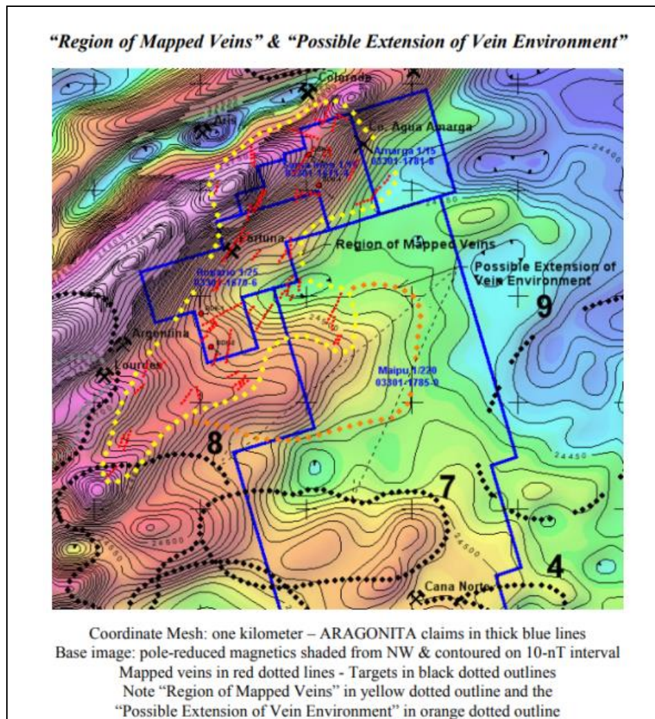
Figure 5 Possible Extension of Vein Environment Target (Ludwig 2009)
