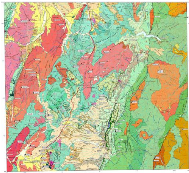
Figure 6 Regional Geological Setting (Arévalo et. al. 2009)
