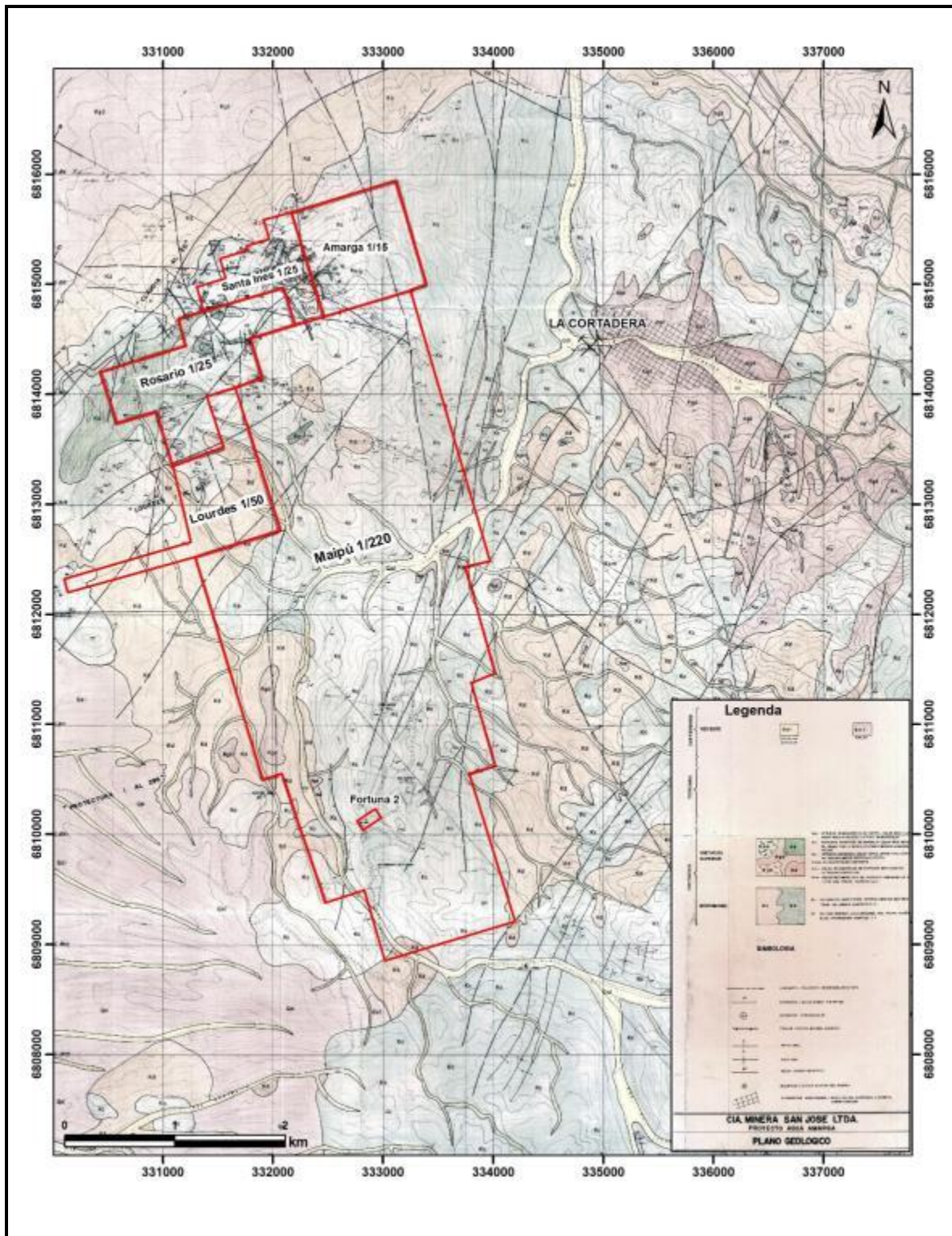
Figure 7 Geology of the Agua Amarga Property (Carmichael 1983)
