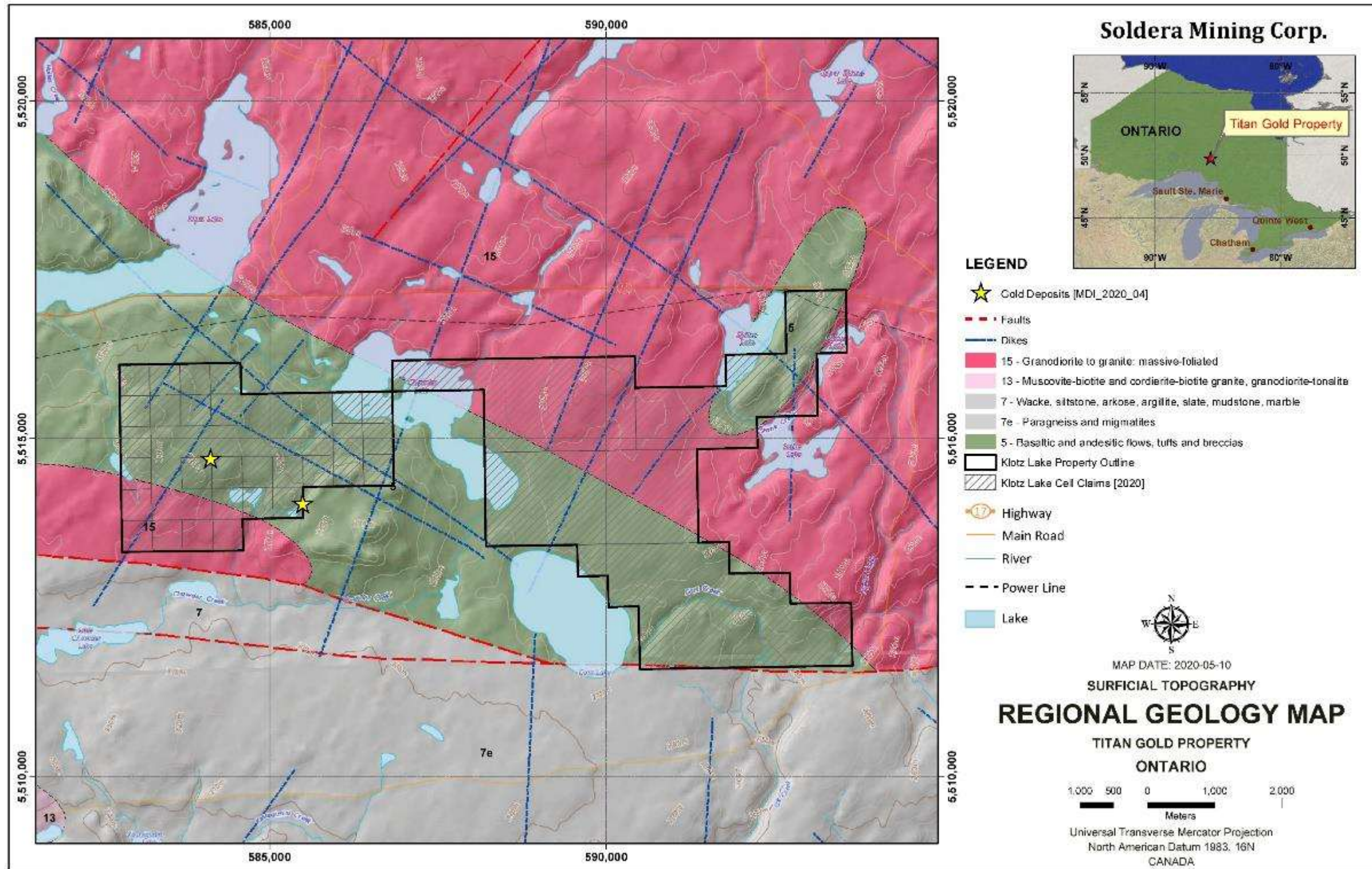
Figure 17: Property Geology Map
