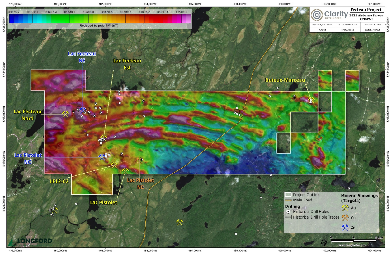
Figure 1 Fecteau Property preliminary results showing RTP-TMI from recently completed airborne Triaxial Magnetometer survey.
