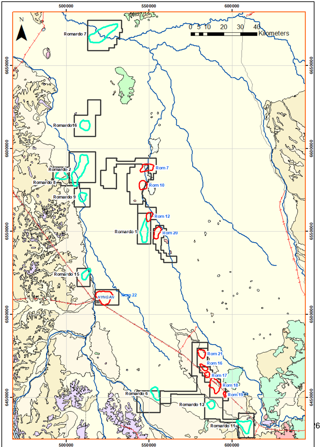
Figure 8: Property Geology
