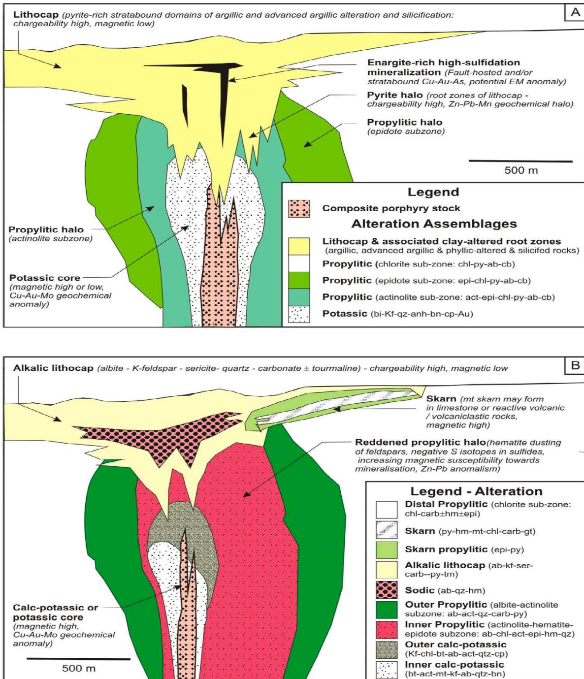
Figure 9: Deposit Model
