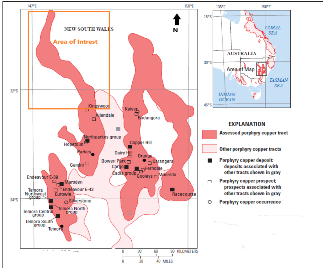
Figure 7: Macquarie Extension
