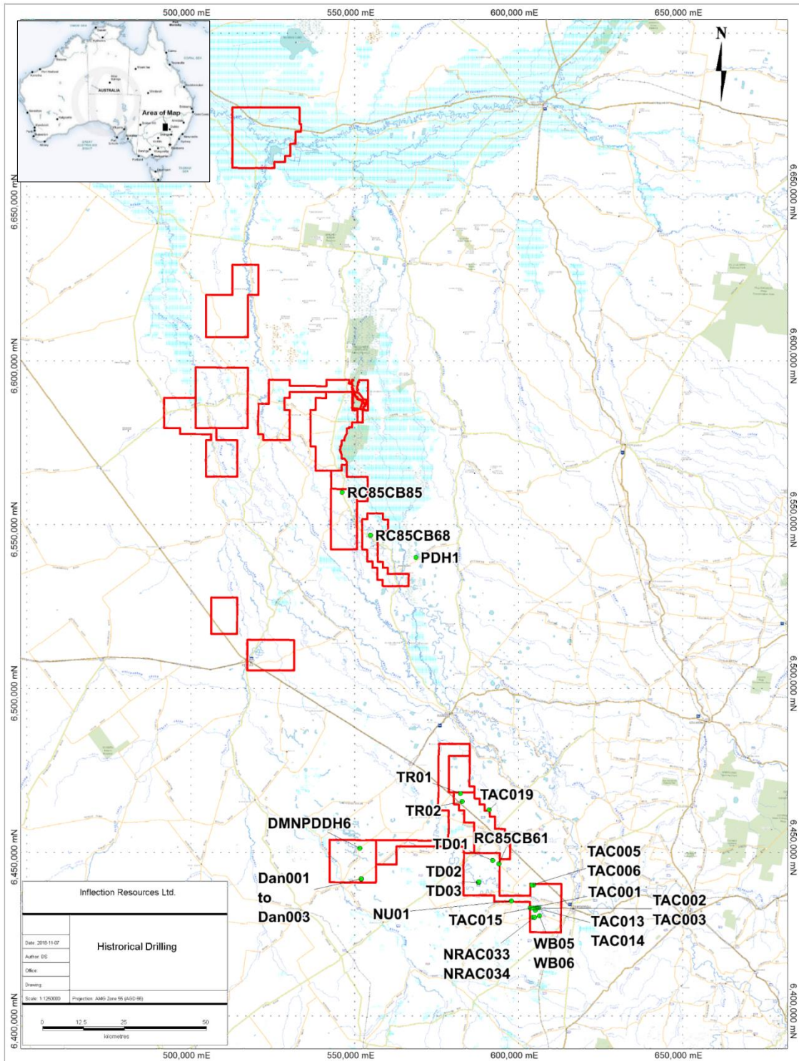
Figure 2: Historical Drilling
