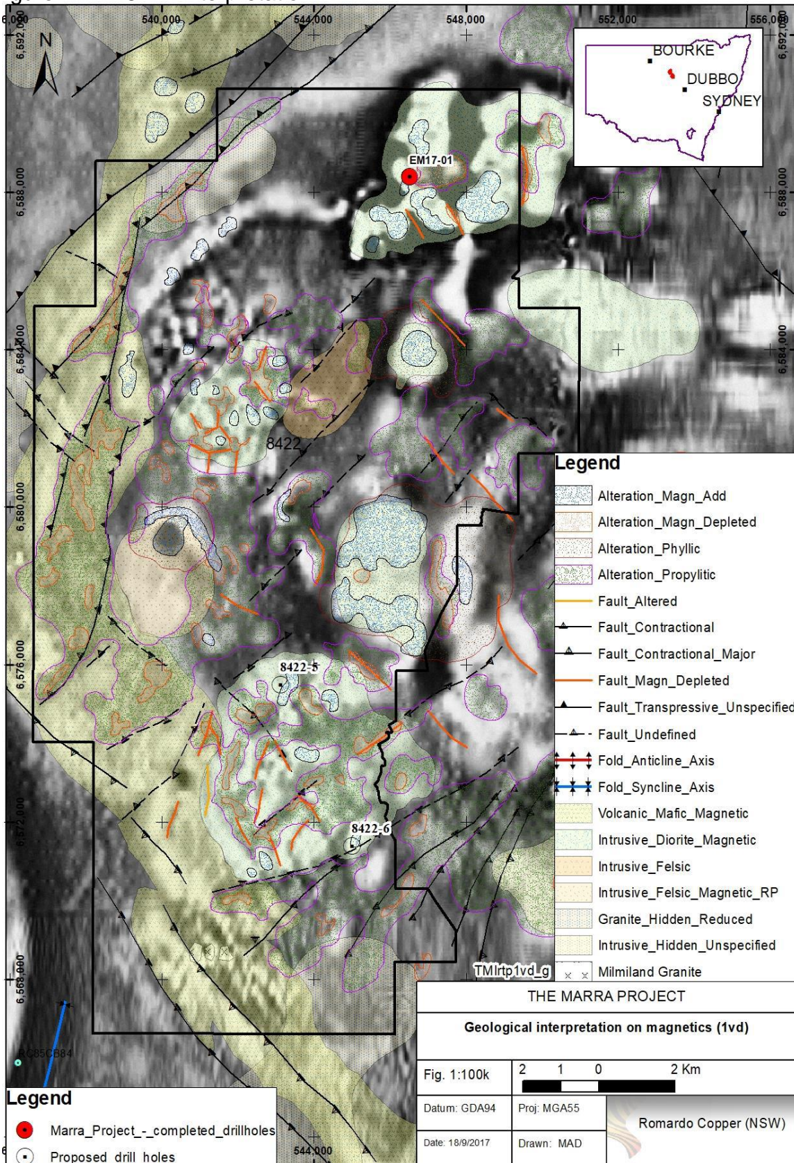
Figure 4: EL 8422 Interpretation
