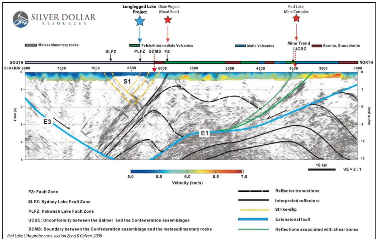
Figure 6: Deep Penetrating Regional Lithoprobe Seismic Survey
