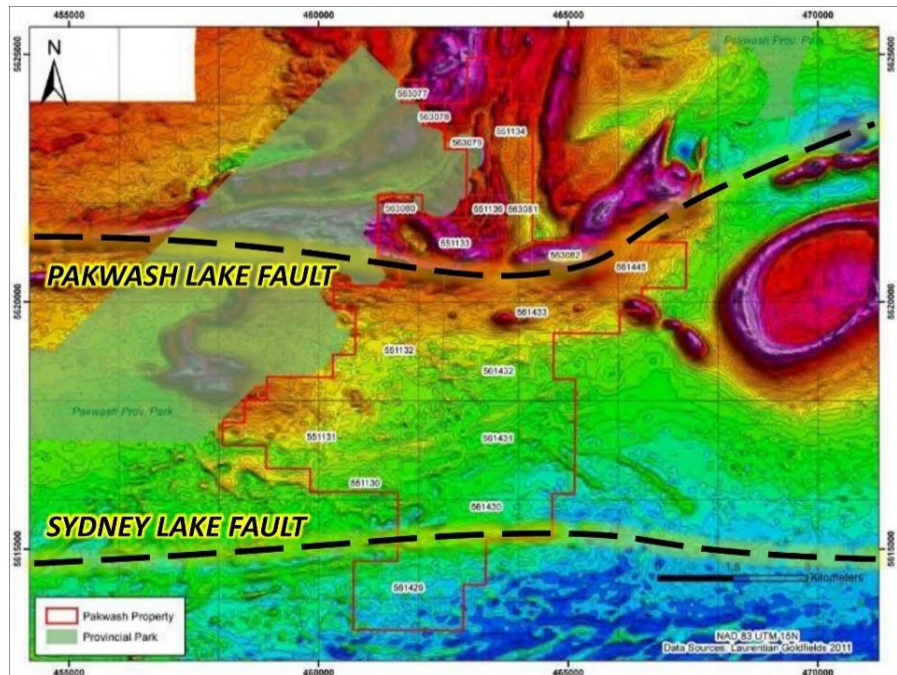
Figure 8: 2011 MAG Survey with Interpreted Tracing of the PLFZ and SLFZ Structures Crossing the Property
