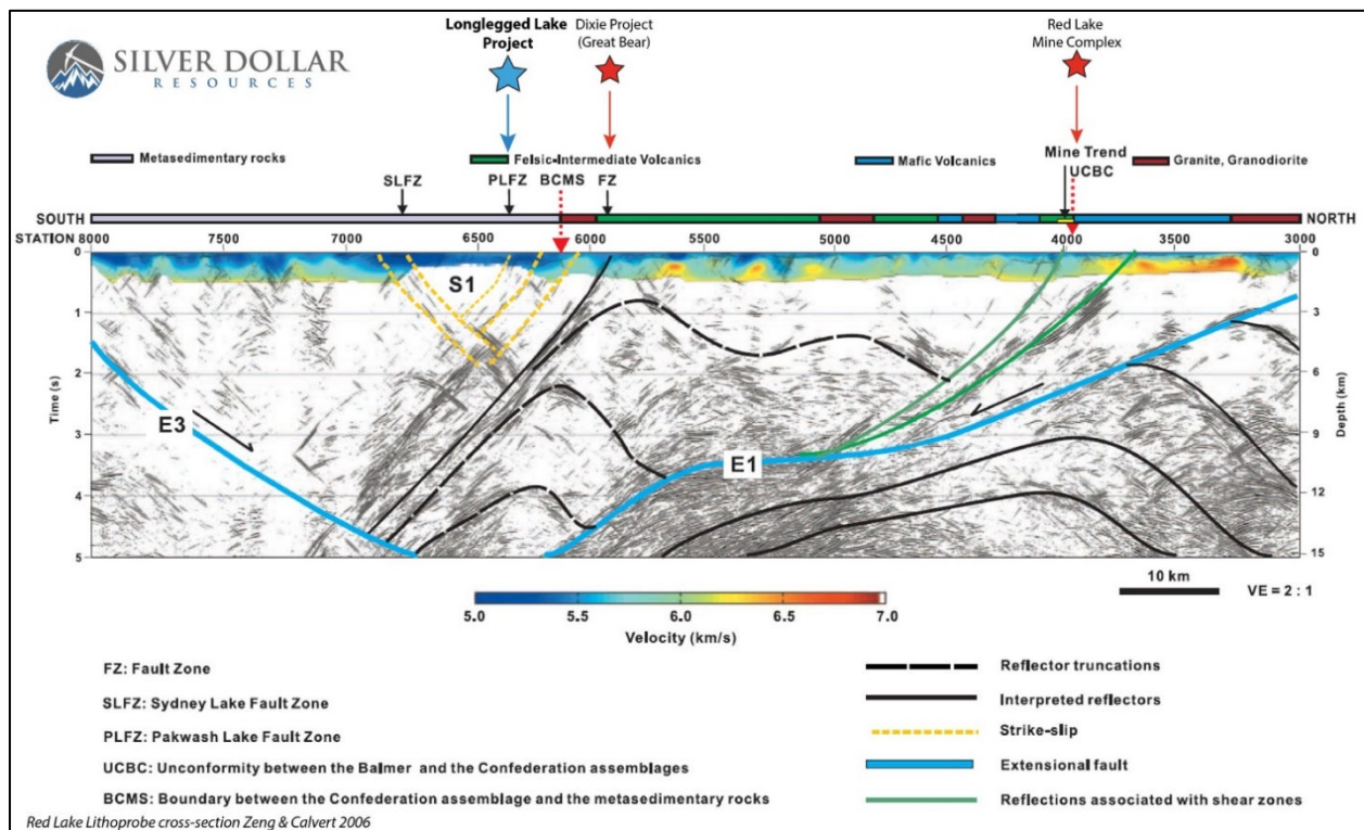
Figure 6: Deep Penetrating Regional Lithoprobe Seismic Survey
