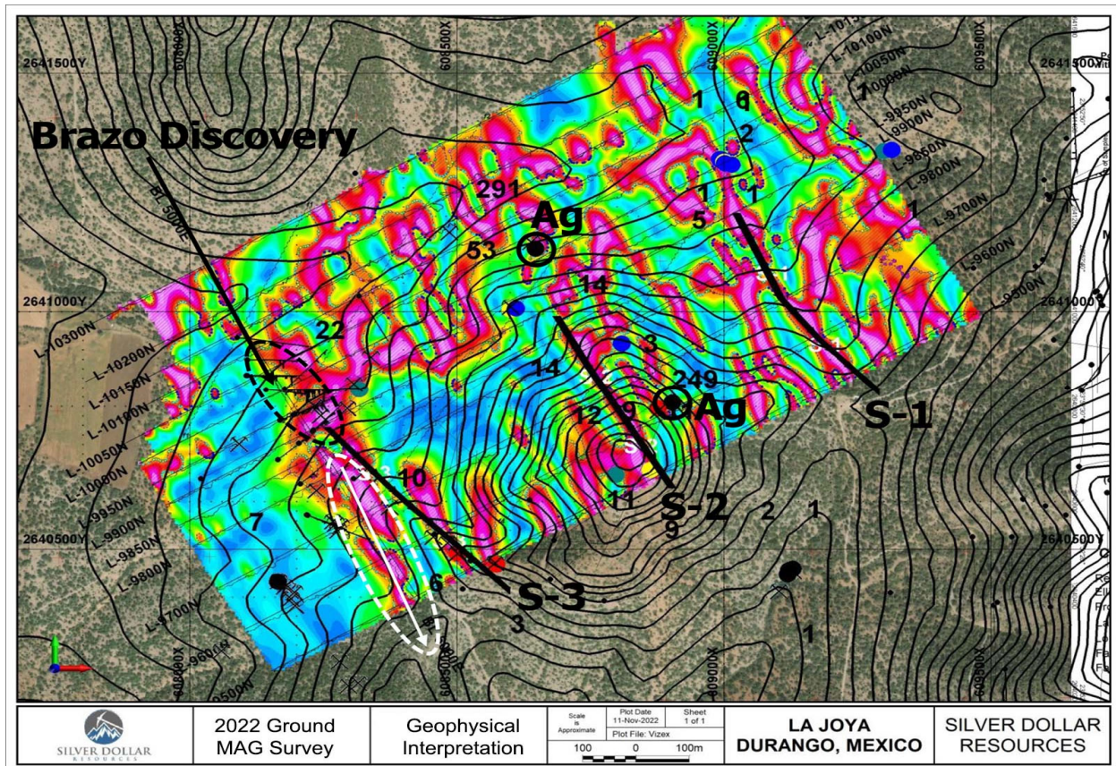
Figure 5: 2022 Brazo Discovery ground magnetic survey and geophysical interpretation
