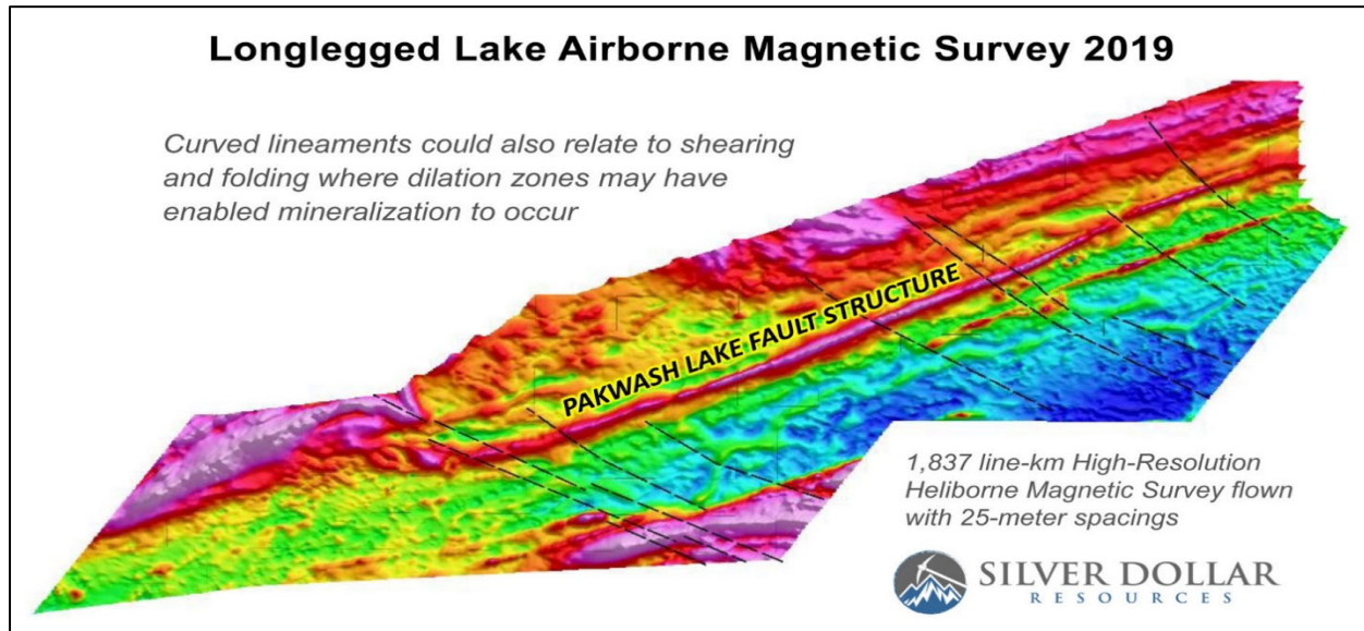
Figure 6: MAG Survey Showing Pakwash Lake Fault Zone Structure and Curved Lineaments
