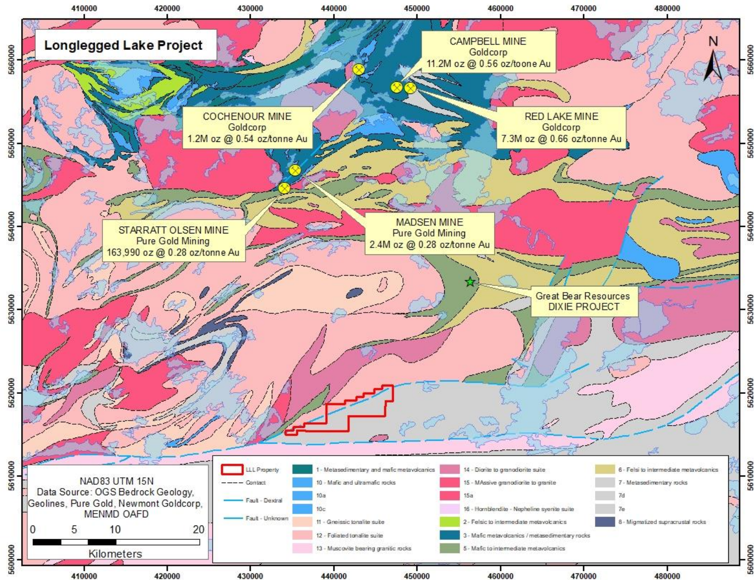
Figure 3. Regional Geology
