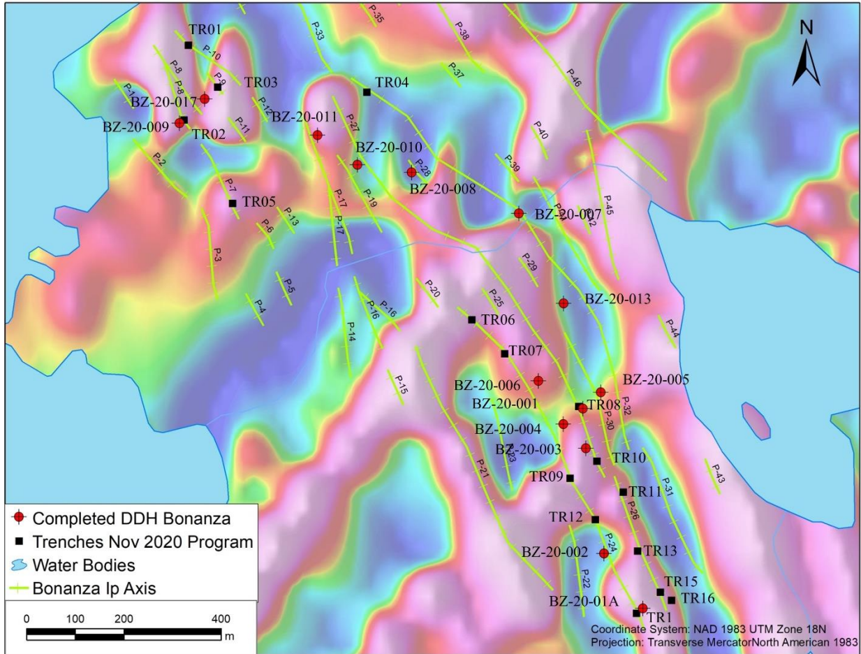
Figure 1. Location of Trenches and DDH, over FVD. Please note that two trenches are located further south and are not shown on this map for simplicity reasons.
