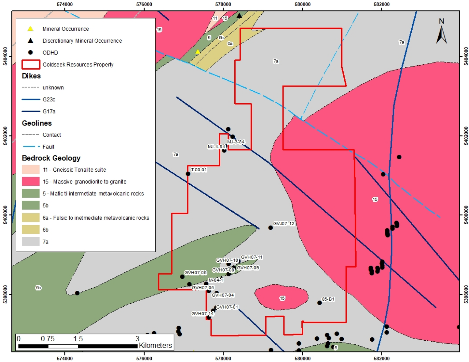
Figure 4: Horizon Property Geology
