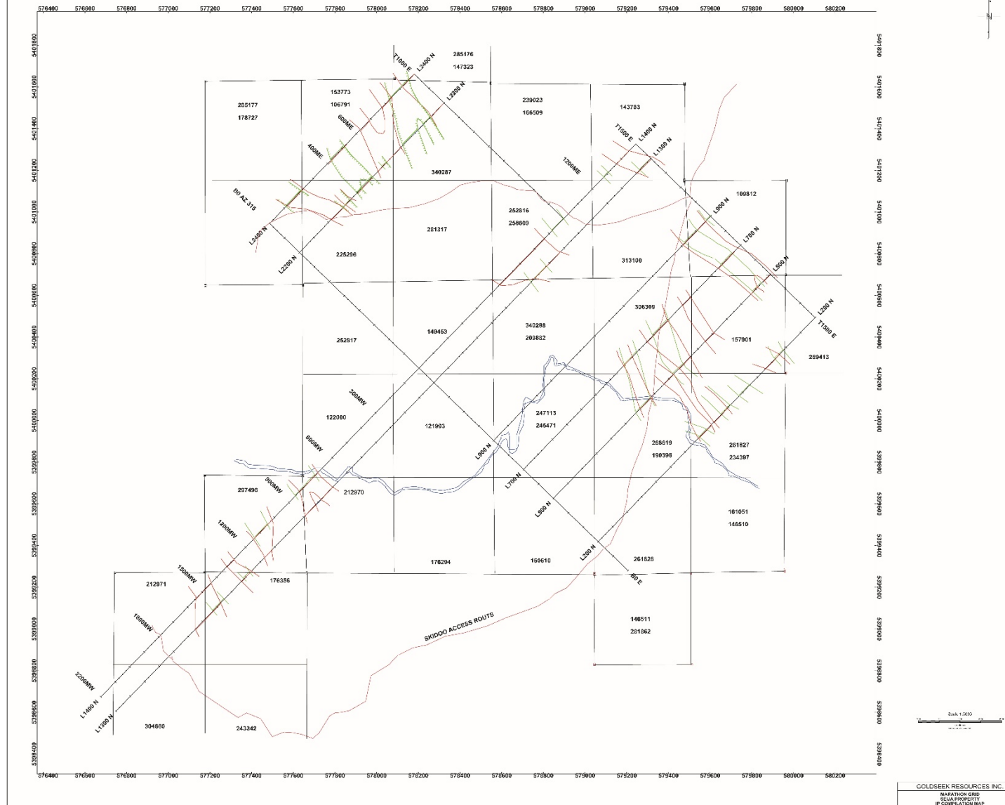
Figure 5: Goldseek 2019 IP Survey Grid
