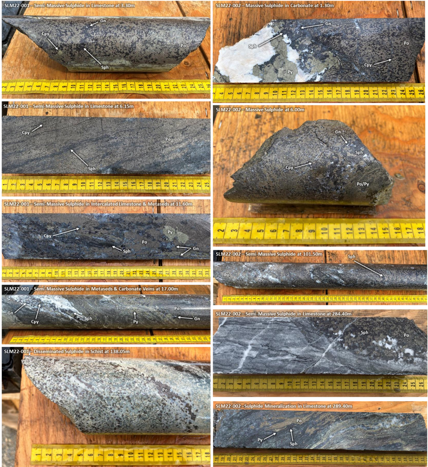
Figure 1: Photographs of representative 2022 HQ-sized core intervals from SLM22-001 and SLM22-002 of base metal sulphide (Chalcopyrite = Cpy; Galena = Gn; Sphalerite = Sph; Pyrrhotite = Po; Pyrite = Py) occurrences at the Jackie Target, Silver Lime Project.
