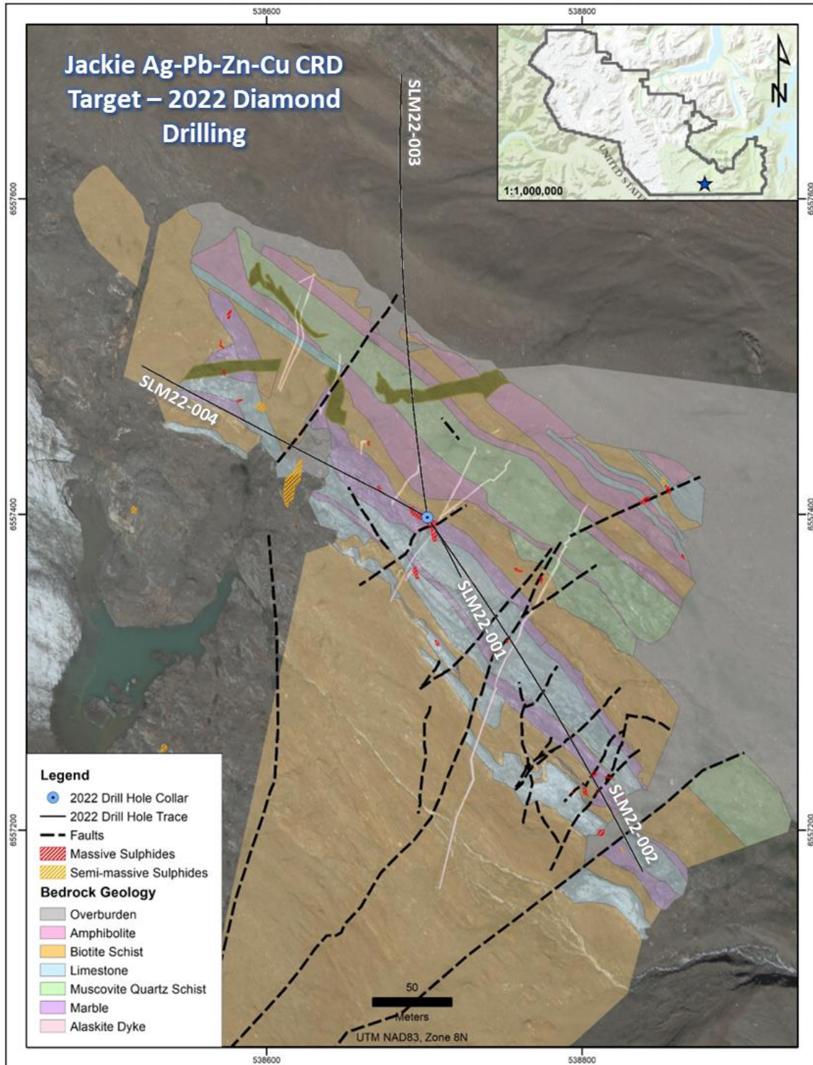
Figure 3: Planview geology map of the Jackie Target at the Silver Lime Project showing 2022 diamond drilling progress and mapped massive to semi massive sulphide occurrences.
