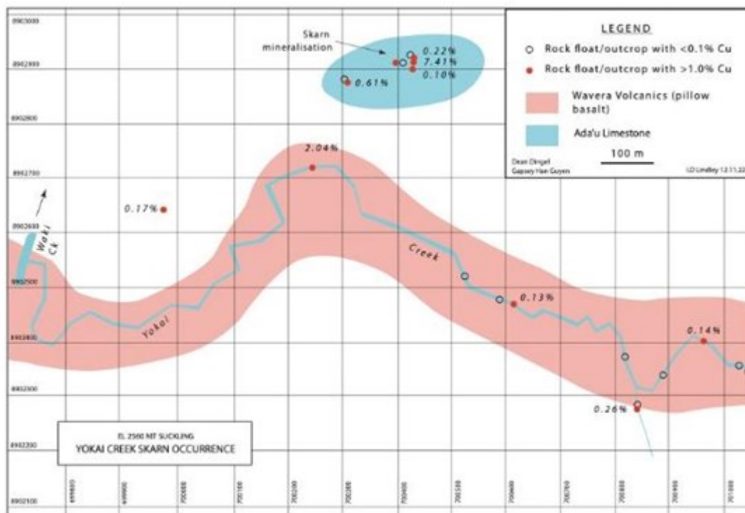
Figure 1: Reconnaissance sampling of lower Yokai creek, southeast Urua-Omu project area.
