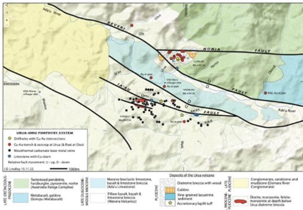
Figure 2: Geological map of the Urua-Omu project area, showing three distinct tectonic blocks, viz. Urua, Yokai and Omu blocks, each with different erosional levels and contrasting porphyry potential, necessitating unique approaches to exploration.
