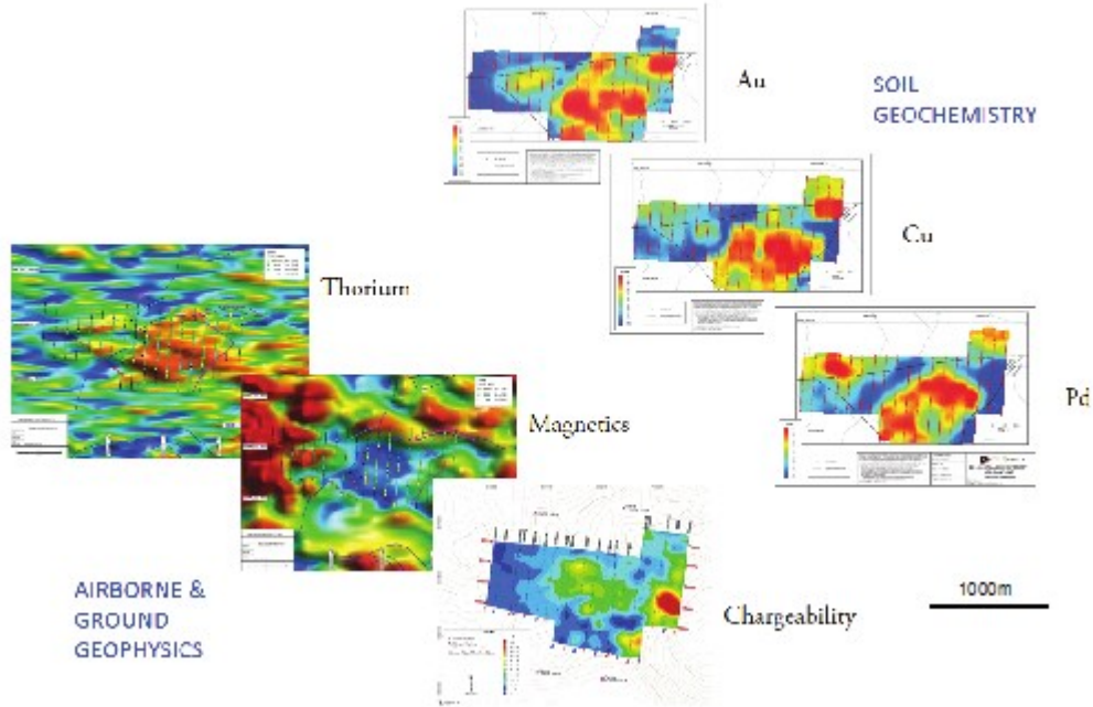
Figure 3: Urua with its coincident Au-Cu-Pd soil geochemistry, airborne geophysical signatures (thorium and magnetics) and chargeability.
