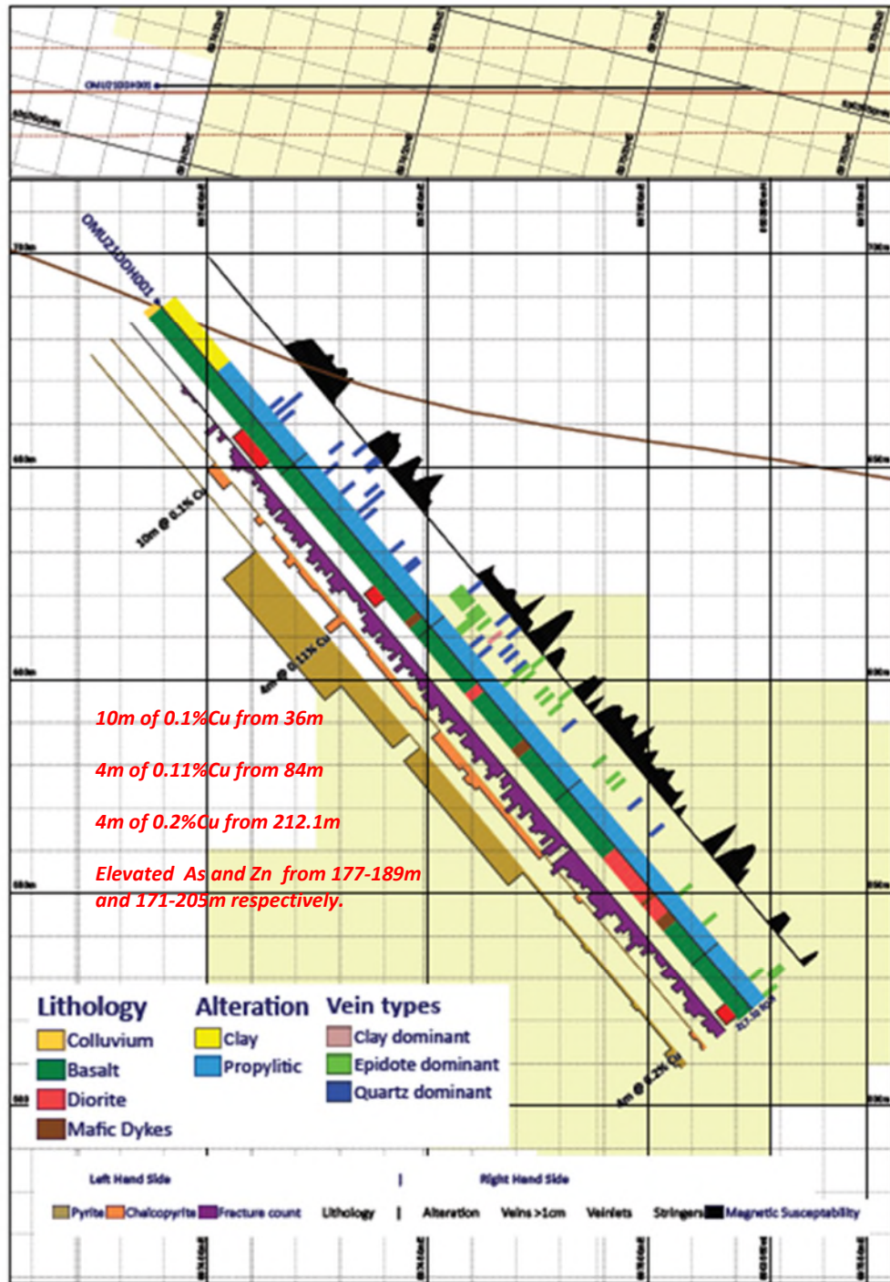
Figure 3. Geological section of drill hole OMU21DD001 showing the distribution of chalcopyrite mineralization associated with quartz-epidote-pyrite veins.
