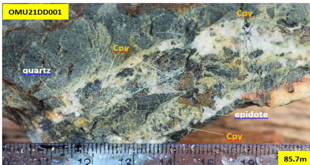
Figure 2. Coarse-grained chalcopyrite associated with quartz and epidote veins at 85.7m depth. (0.12%Cu from 84-86m)
