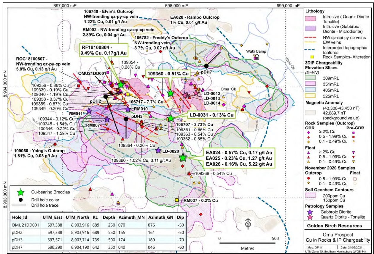
Figure 5. Location of the Cu-bearing breccias (green stars) illustrating a NNW (north-northwest) trend.
