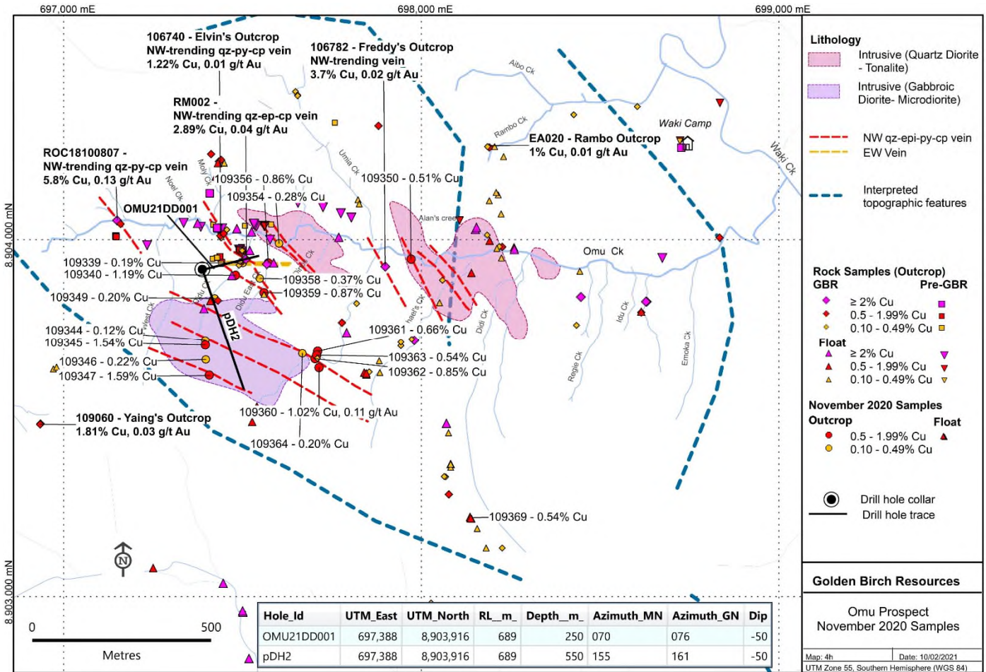
Figure 1. Location of Omu rock samples collected in November 2020.
