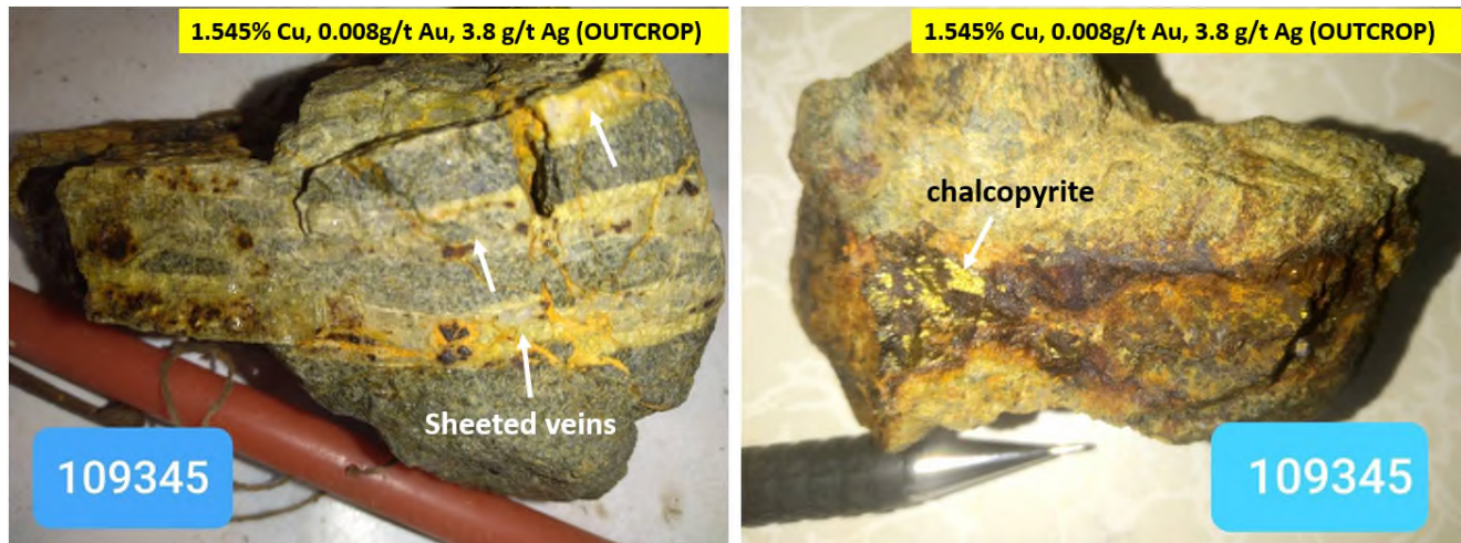
Figure 2. Left: Outcrop sample of fine-grained diorite at the headwaters of Didu creek showing sheeted veins with oxides (after chalcopyrite). Right: Different view of the same sample showing chalcopyrite blebs in fracture.
