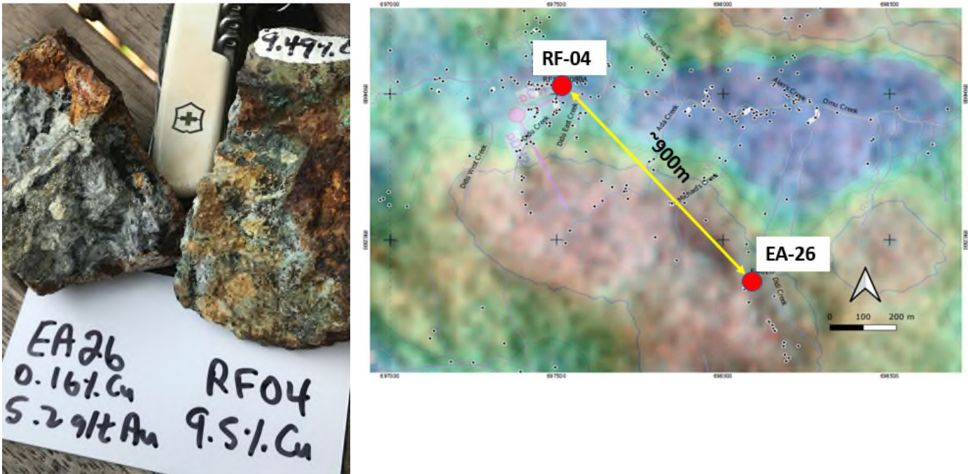
Figure 3. EA-26 and RF-04 blocky float samples (left image) demonstrating strong similarities in appearance, alteration, mineralization and petrologic descriptions. These samples (~900m apart) maybe part of a large system and provide even further evidence of a strongly mineralised and potentially high grade copper zone at Omu prospect.
