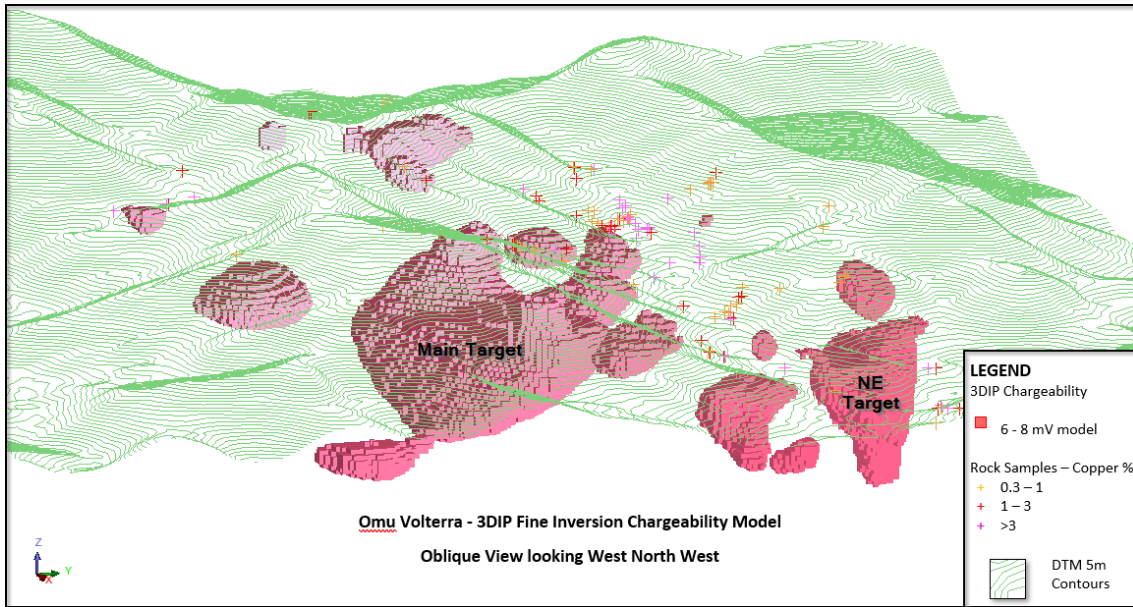
Figure 10: 3D image of modelled IP results. Targets open at depth given the constraints of the survey below 400 metres.
