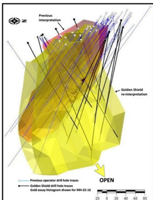
Figure 4. Three-dimensional view showing current and previous interpretations of QMC host rock unit and historic and Golden Shield drill holes. (CNW Group/Golden Shield Resources)
