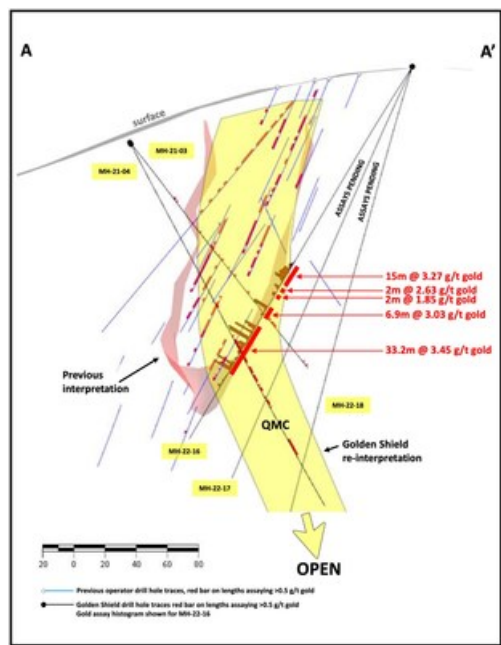
Figure 3. Cross section (A-A') showing previous and current interpretations of QMC host rock and historic and golden shield drill holes. (CNW Group/Golden Shield Resources)
