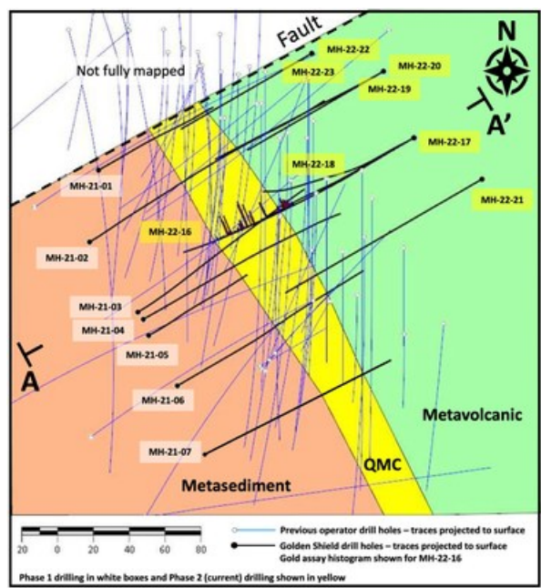
Figure 2. Mazoa Hill surface geology map with historic drilling and completed Golden Shield drill hole locations (CNW Group/Golden Shield Resources)
