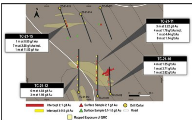
Figure 2 – Toucan Creek drill plan with mapped geology and surface sample results. (CNW Group/Golden Shield Resources)
