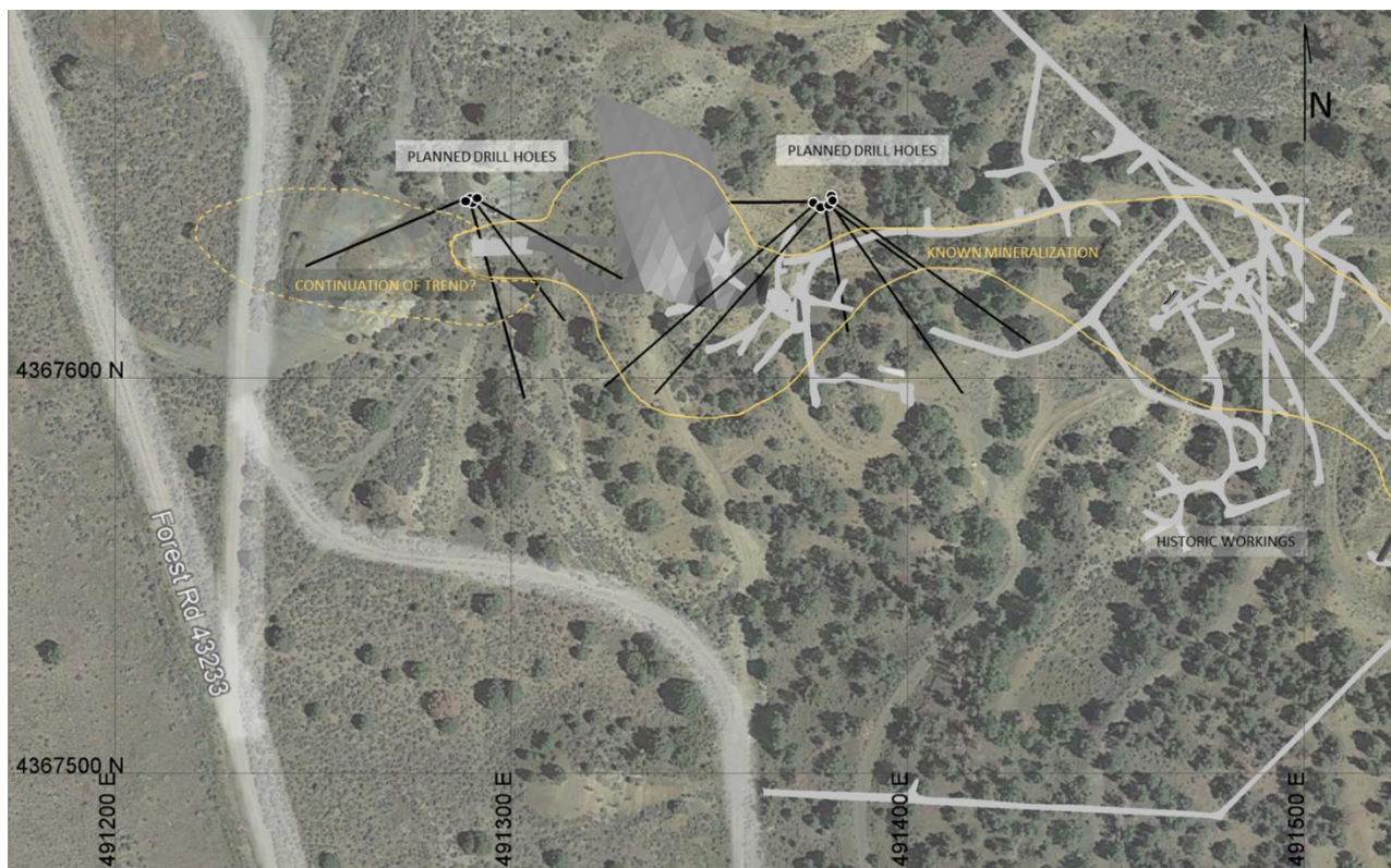
Figure 1. Proposed Drill Hole Locations at the Apex Property
