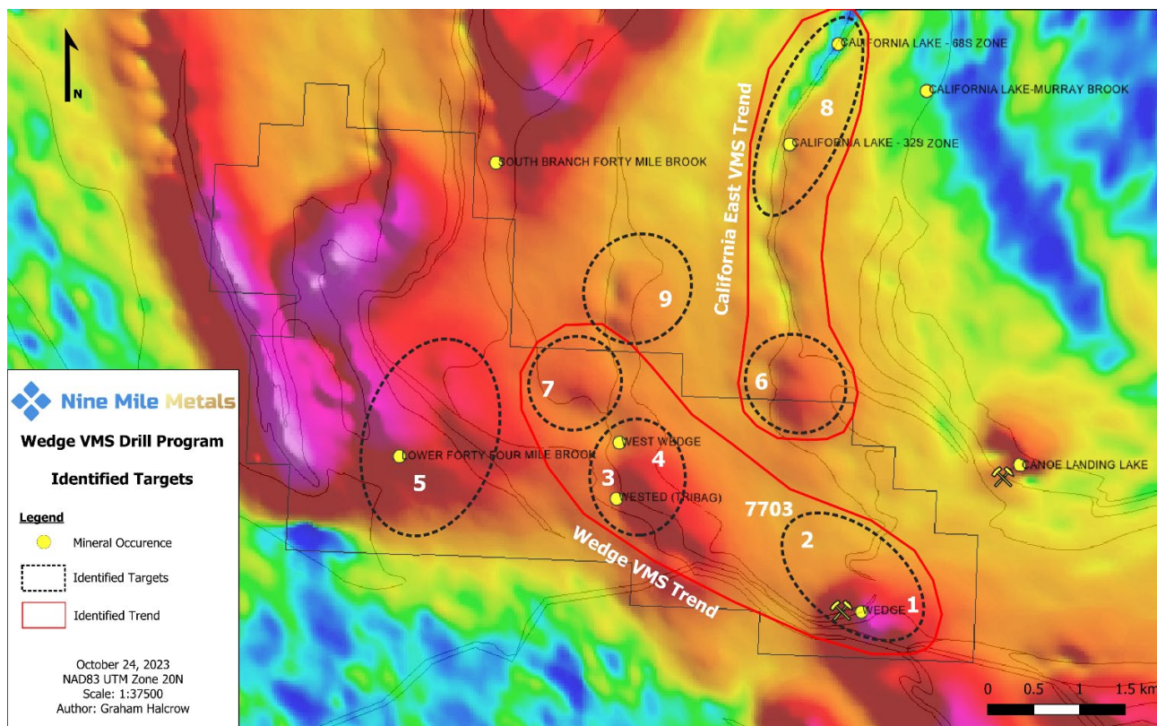
Figure 4 - "New" Drill Program High Priority Targets, Wedge Project Area, New Brunswick
