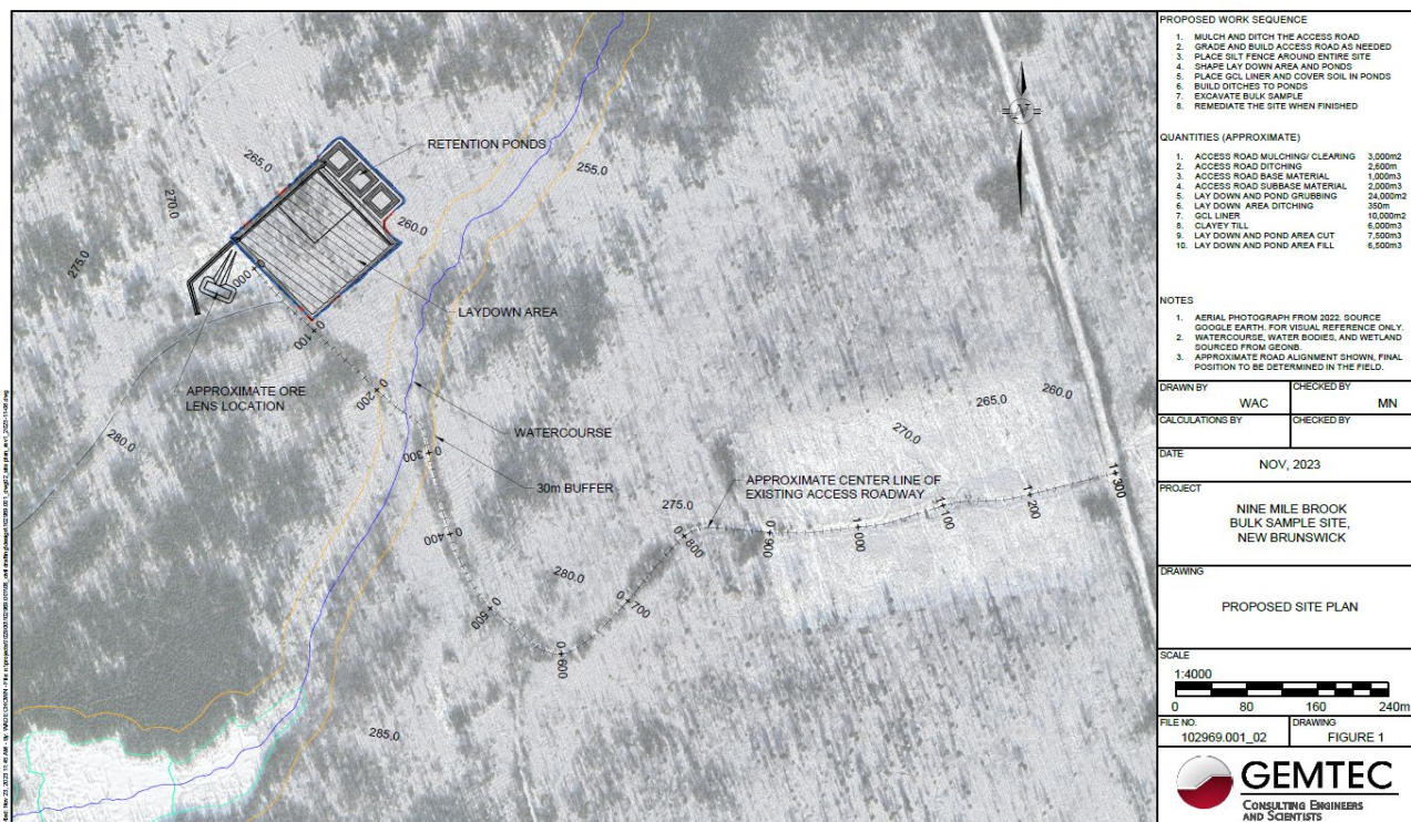
Figure 3 – Nine Mile Brook Lens Bulk Sample Site Plan
