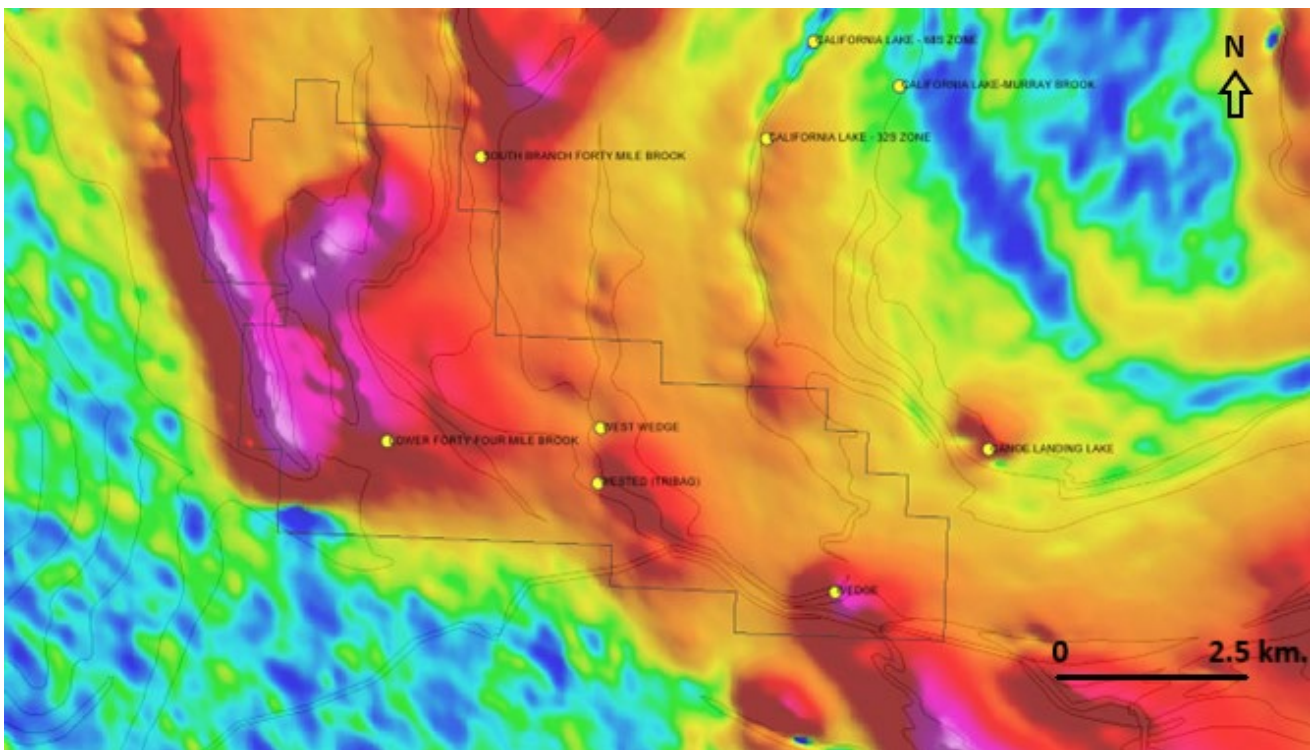
Figure 1: Newly acquired Wedge property displaying EarthEX reprocessed TDEM data with targets.
