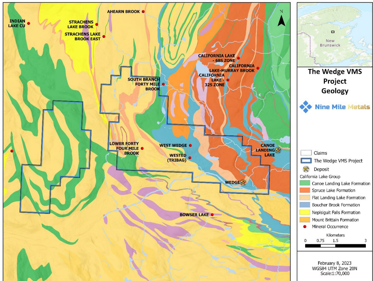
Figure 2: The new “Wedge VMS Project” Geology
