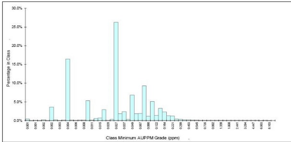
Bullfrog : frequency distribution of AUPPM in BF-Background : raw assays
