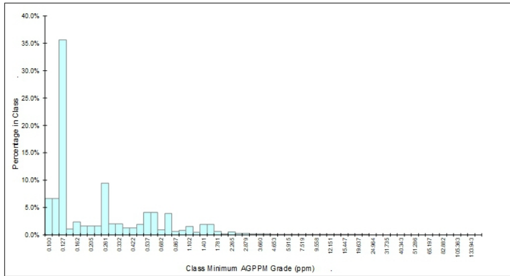
Bullfrog : frequency distribution of AGPPM in BF-Background : raw assays
