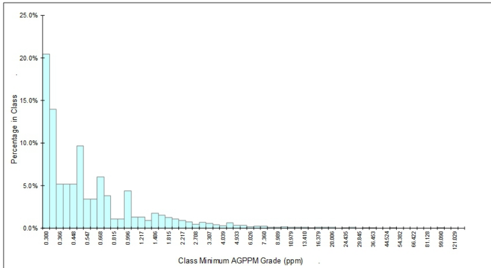
Bullfrog: frequency distribution of AGPPM in MS-Background: raw assays
