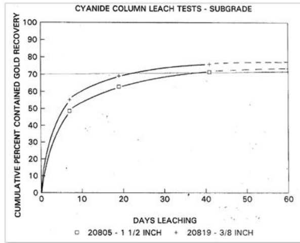
Figure 10-1: Leach Test Results
