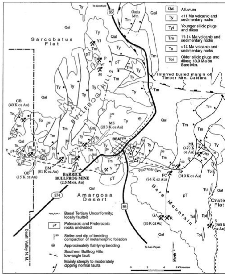
Figure 1-2: District Geology Map
