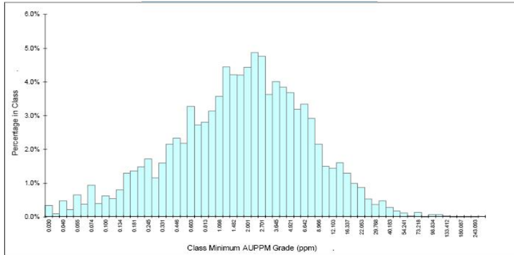
Bullfrog : frequency distribution of AUPPM in BF-Vein : raw assays
