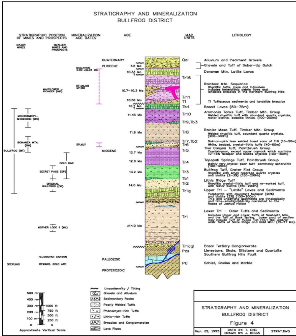
Figure 6-2: Bullfrog District – Stratigraphy and Mineralization
