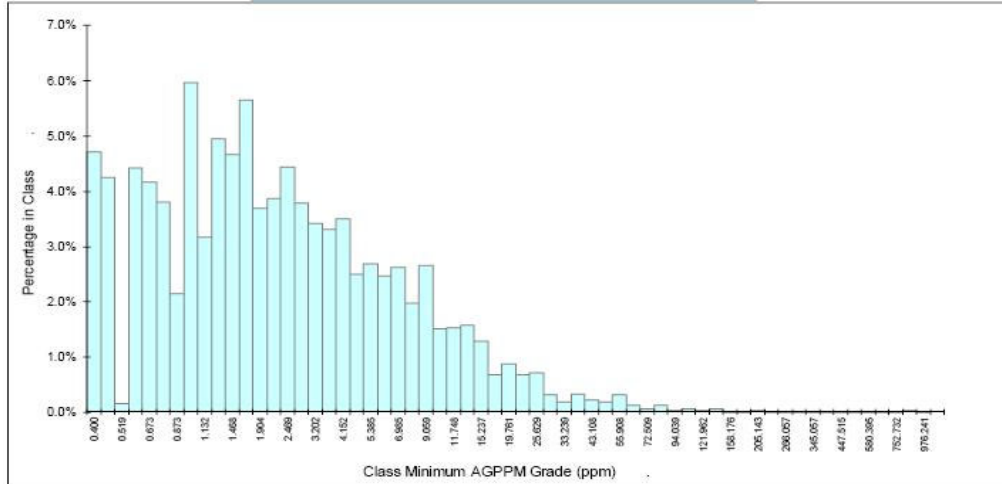
Bullfrog : frequency distribution of AGPPM in MS-Low Grade : raw assays
