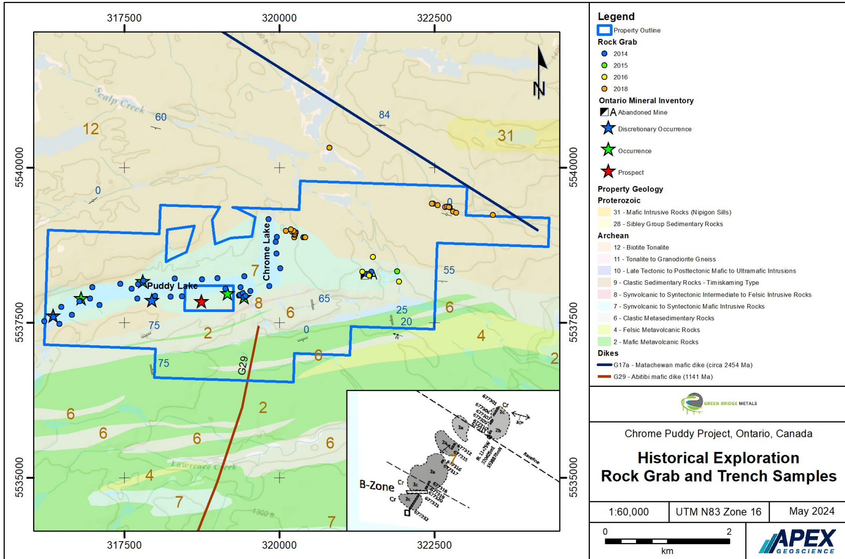
Figure 6.3 Historical exploration conducted by Pavey Ark from 2014 to 2019.
