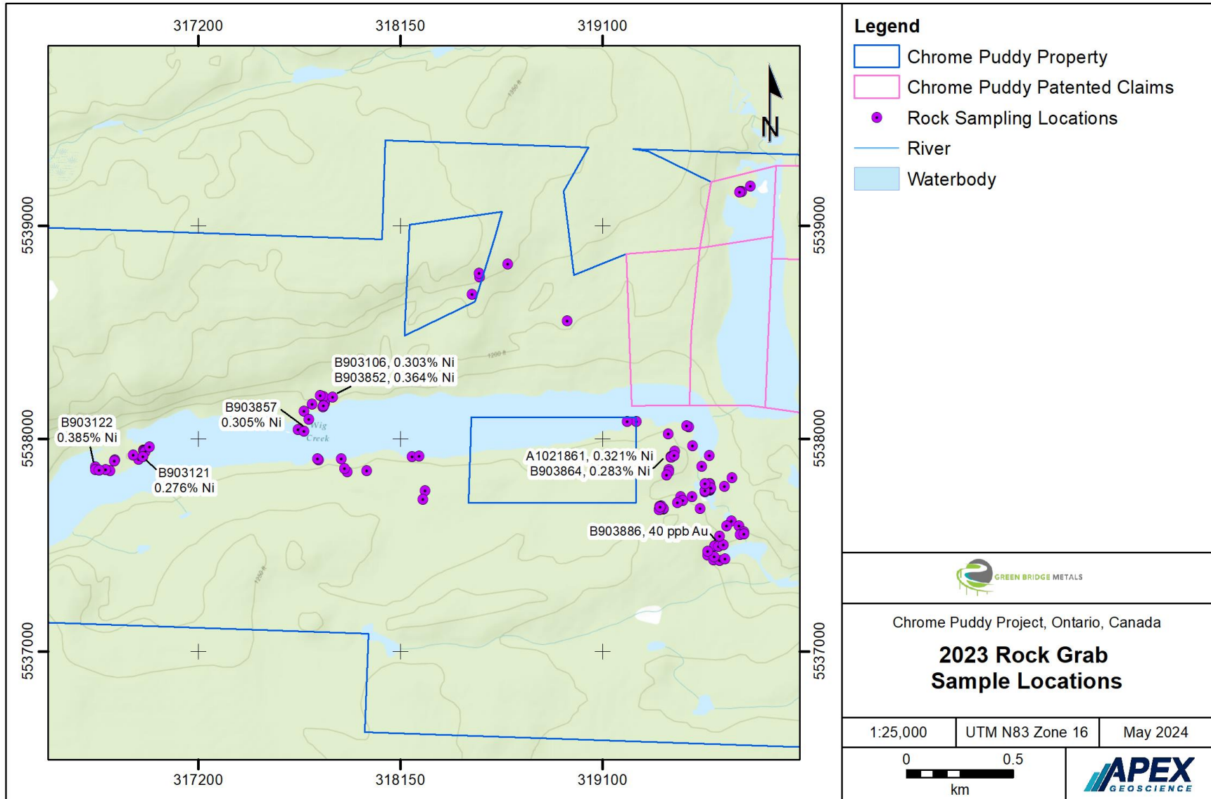
Figure 9.1. 2023 rock sample locations and select geochemical results, Chrome Puddy Property.
