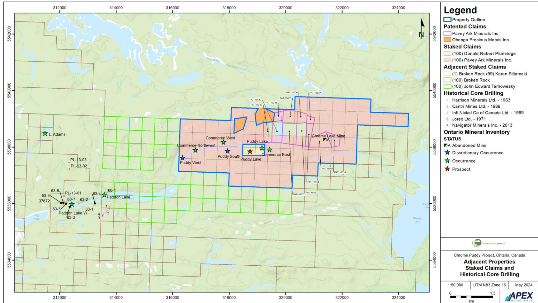
Figure 23.1 Staked claims and historical core drilling adjacent to the Chrome Puddy Property.
