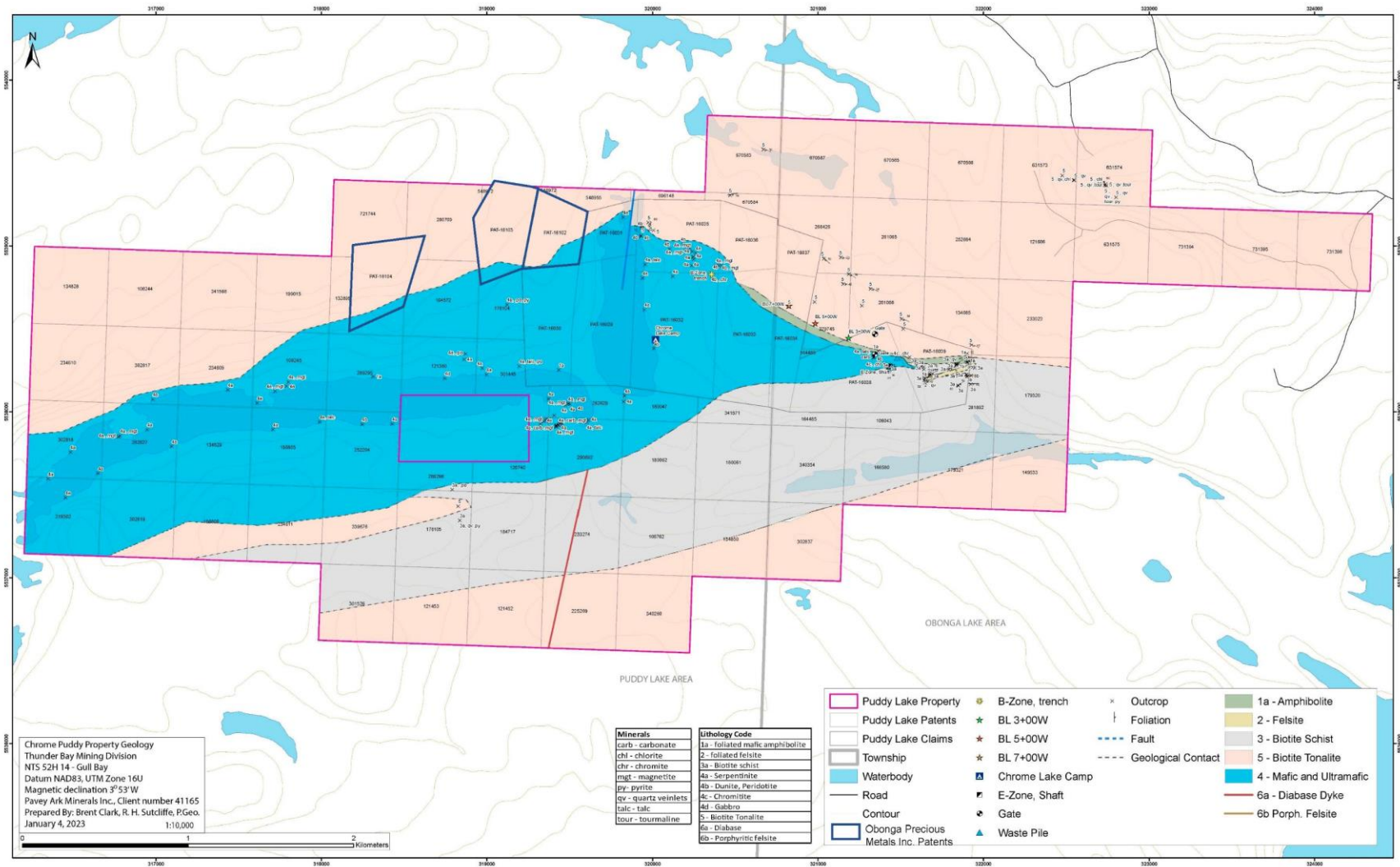
Figure 6.6 Geological mapping completed by Pavey Ark during 2022.
