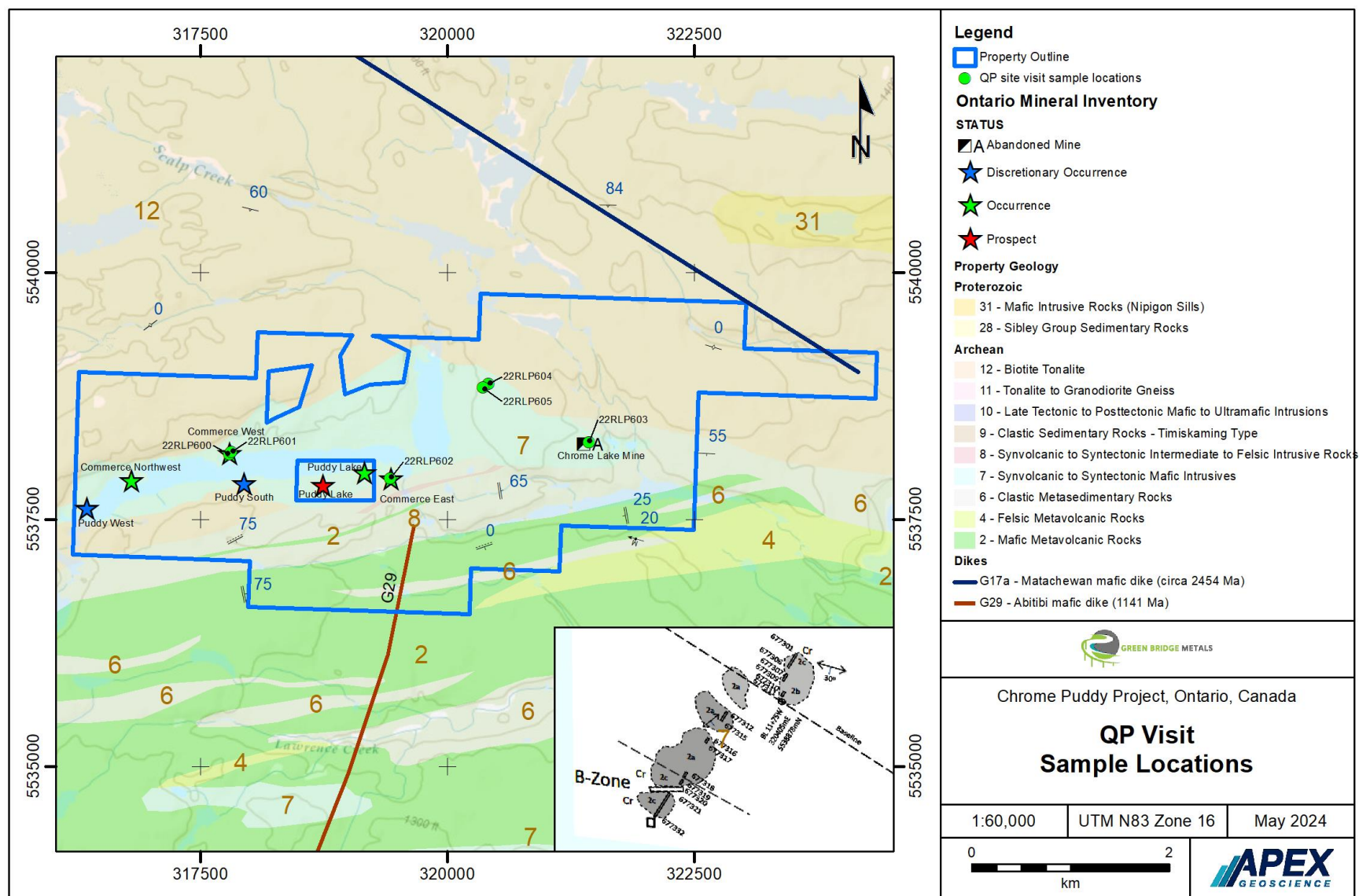
Figure 12.1 QP site inspection sample positions.
