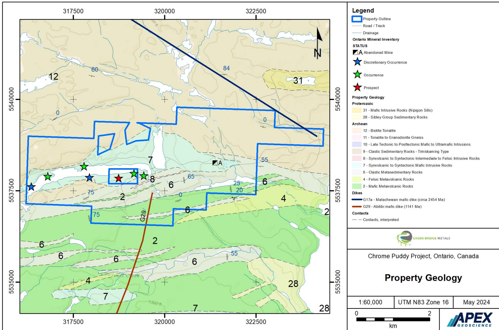
Figure 7.2 Property geology (after Hart, 2006).
