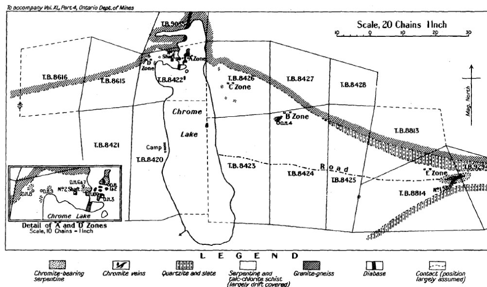
SKETCH MAP SHOWING THE GEOLOGY IN THE VICINITY OF THE CHROMITE DEPOSITS AT CHROME LAKE
