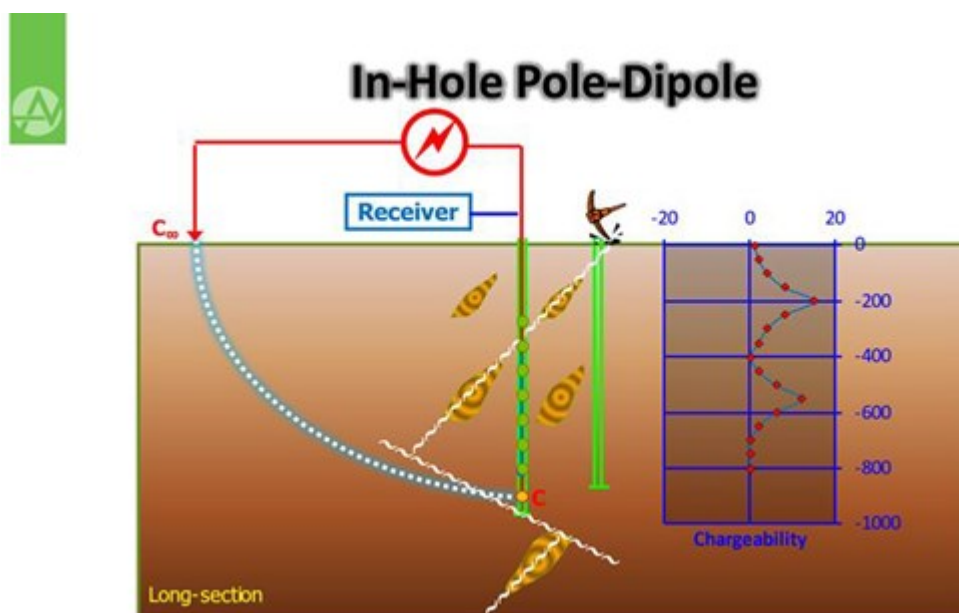
Figure 1. Schematic Diagram of Abitibi Borehole IP
