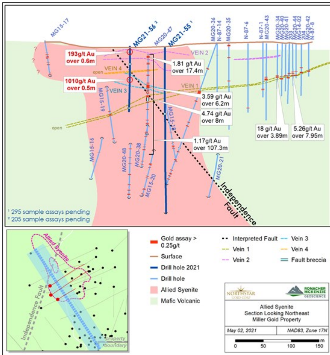
Figure 2. Allied Syenite Cross Section Looking Northeast
